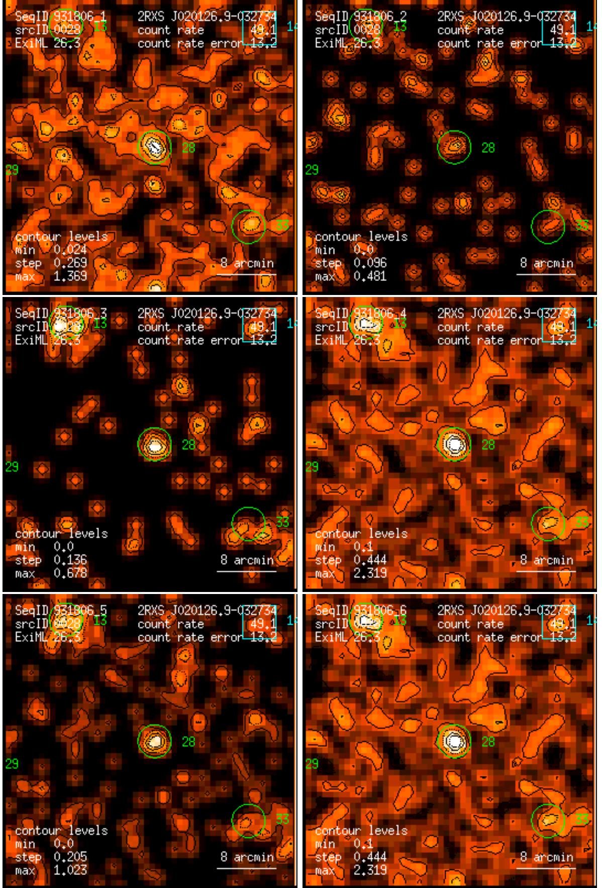
Figure 28: RASS 931806: detection 0028: band rate images, Gaussian filter: (1) PSPC channels 11 – 41, (2) 52 – 90, (3) 91 – 201, (4) 11 – 235, (5) 52 – 201, (6) 11 – 201. Broad band rates in counts/ks. Band rate contour levels in counts/ks/arcmin 2 .
