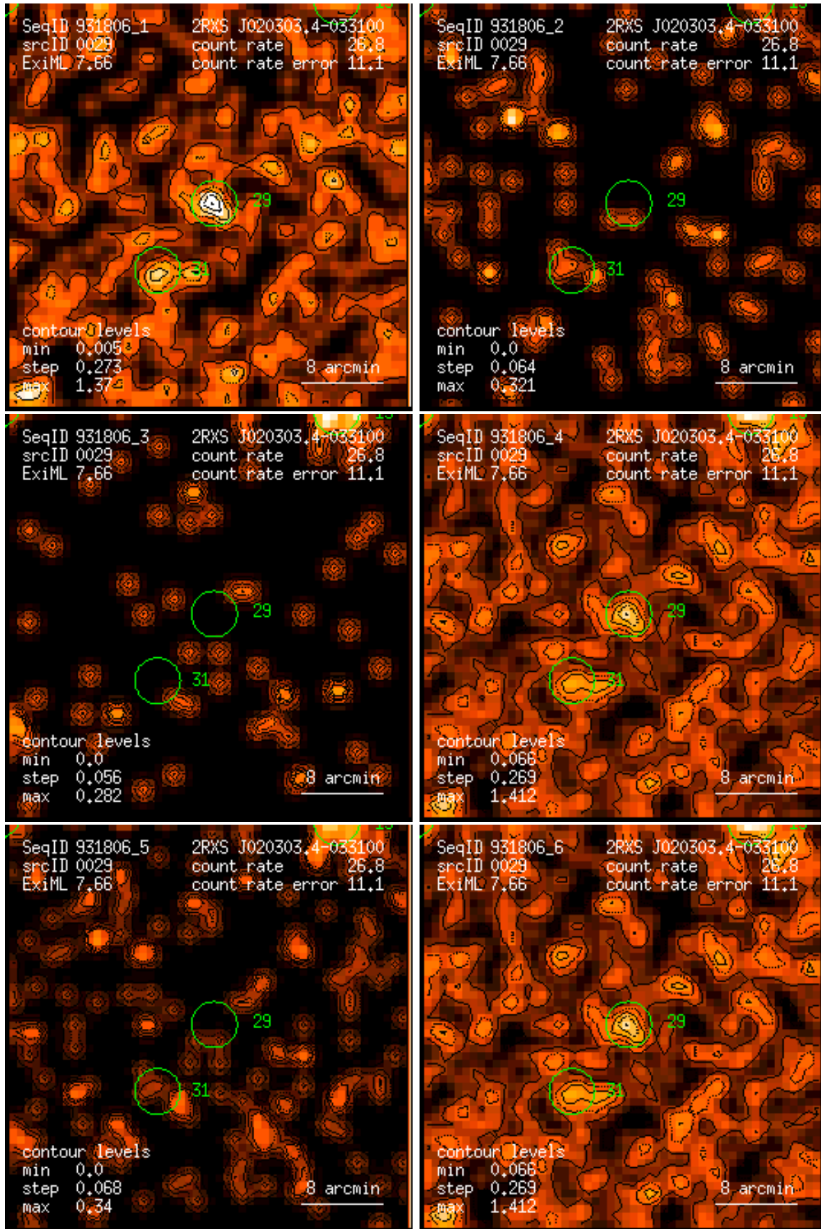
Figure 29: RASS 931806: detection 0029: band rate images, Gaussian filter: (1) PSPC channels 11 – 41, (2) 52 – 90, (3) 91 – 201, (4) 11 – 235, (5) 52 – 201, (6) 11 – 201. Broad band rates in counts/ks. Band rate contour levels in counts/ks/arcmin 2 .
