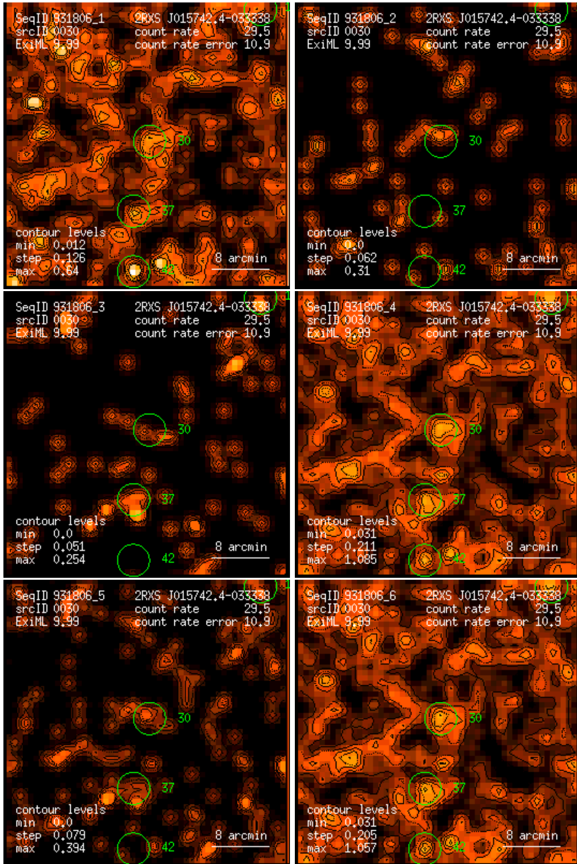
Figure 30: RASS 931806: detection 0030: band rate images, Gaussian filter: (1) PSPC channels 11 – 41, (2) 52 – 90, (3) 91 – 201, (4) 11 – 235, (5) 52 – 201, (6) 11 – 201. Broad band rates in counts/ks. Band rate contour levels in counts/ks/arcmin 2 .
