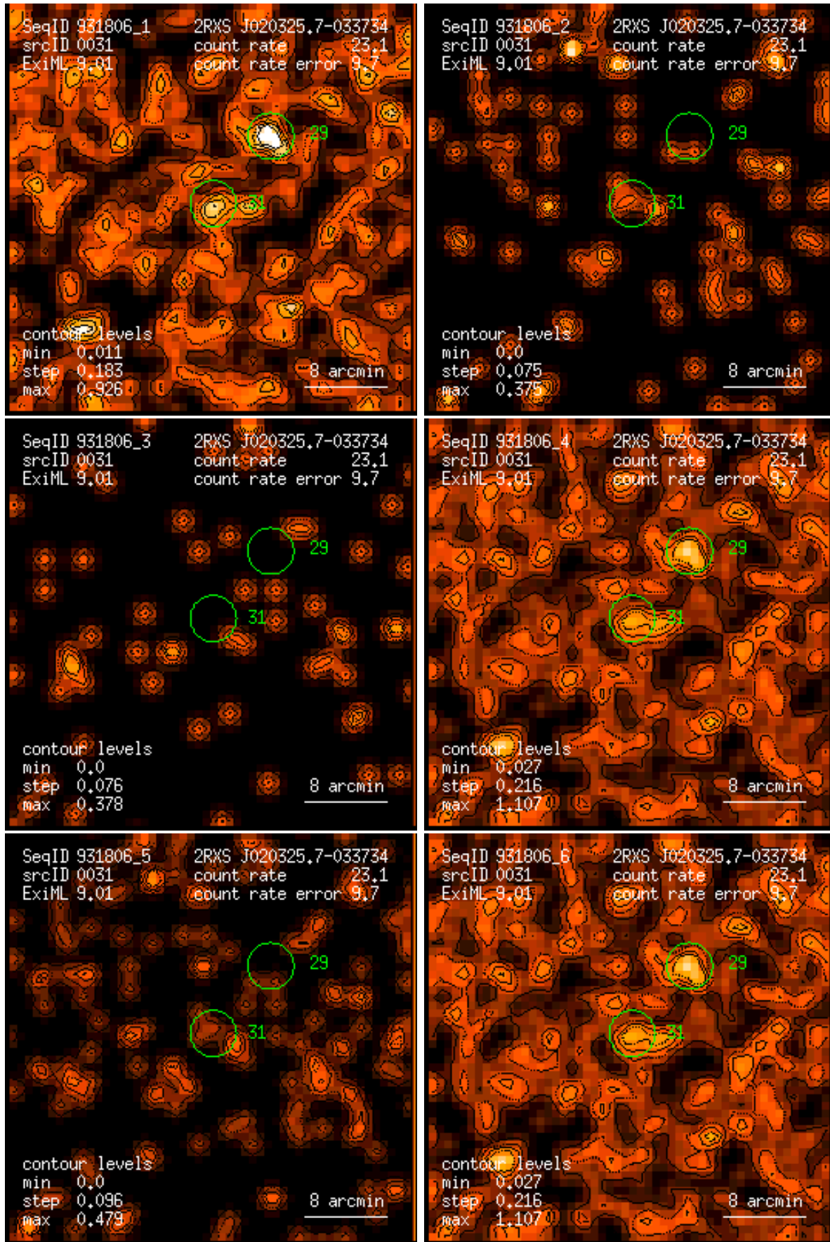
Figure 31: RASS 931806: detection 0031: band rate images, Gaussian filter: (1) PSPC channels 11 – 41, (2) 52 – 90, (3) 91 – 201, (4) 11 – 235, (5) 52 – 201, (6) 11 – 201. Broad band rates in counts/ks. Band rate contour levels in counts/ks/arcmin 2 .
