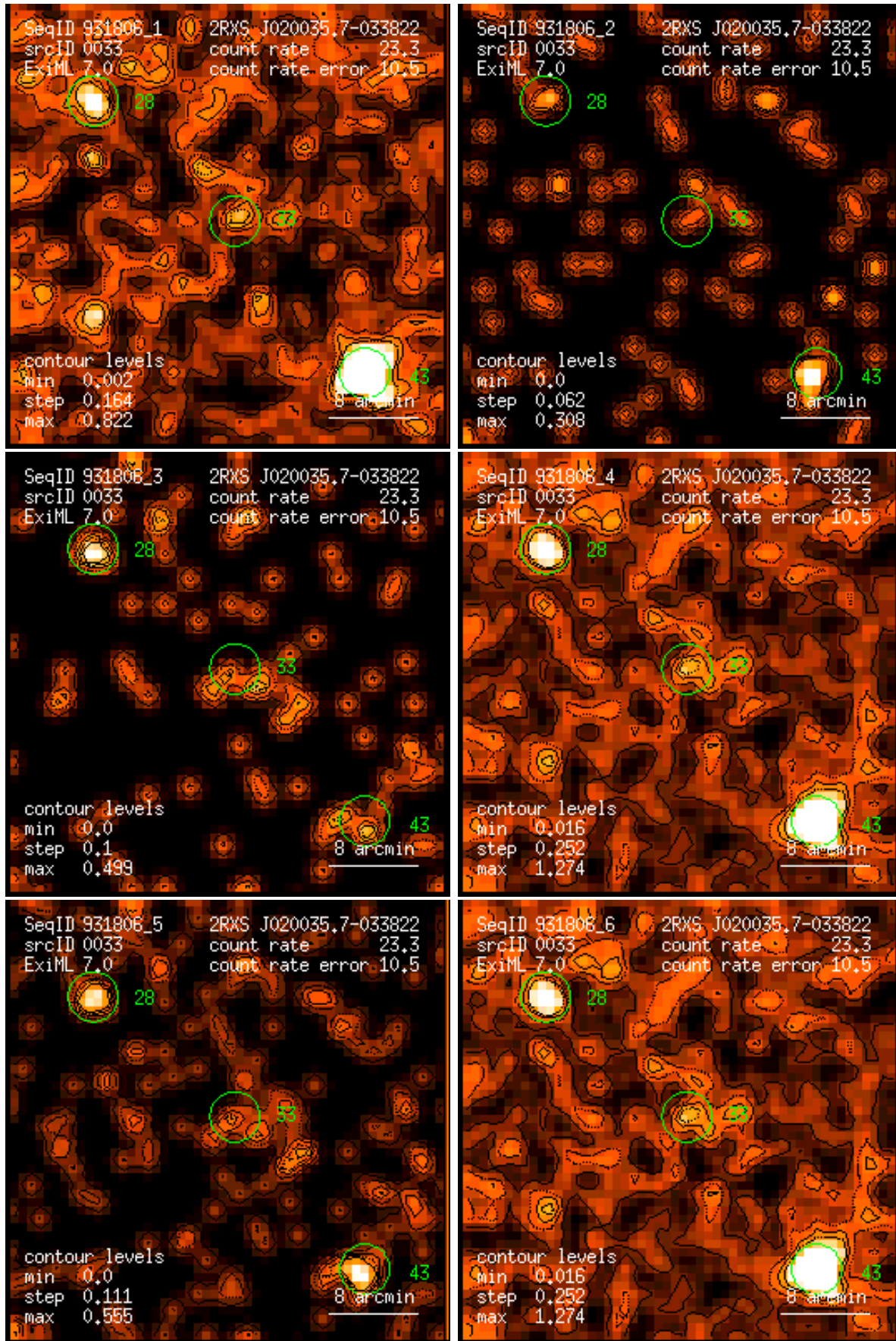
Figure 33: RASS 931806: detection 0033: band rate images, Gaussian filter: (1) PSPC channels 11 – 41, (2) 52 – 90, (3) 91 – 201, (4) 11 – 235, (5) 52 – 201, (6) 11 – 201. Broad band rates in counts/ks. Band rate contour levels in counts/ks/arcmin 2 .
