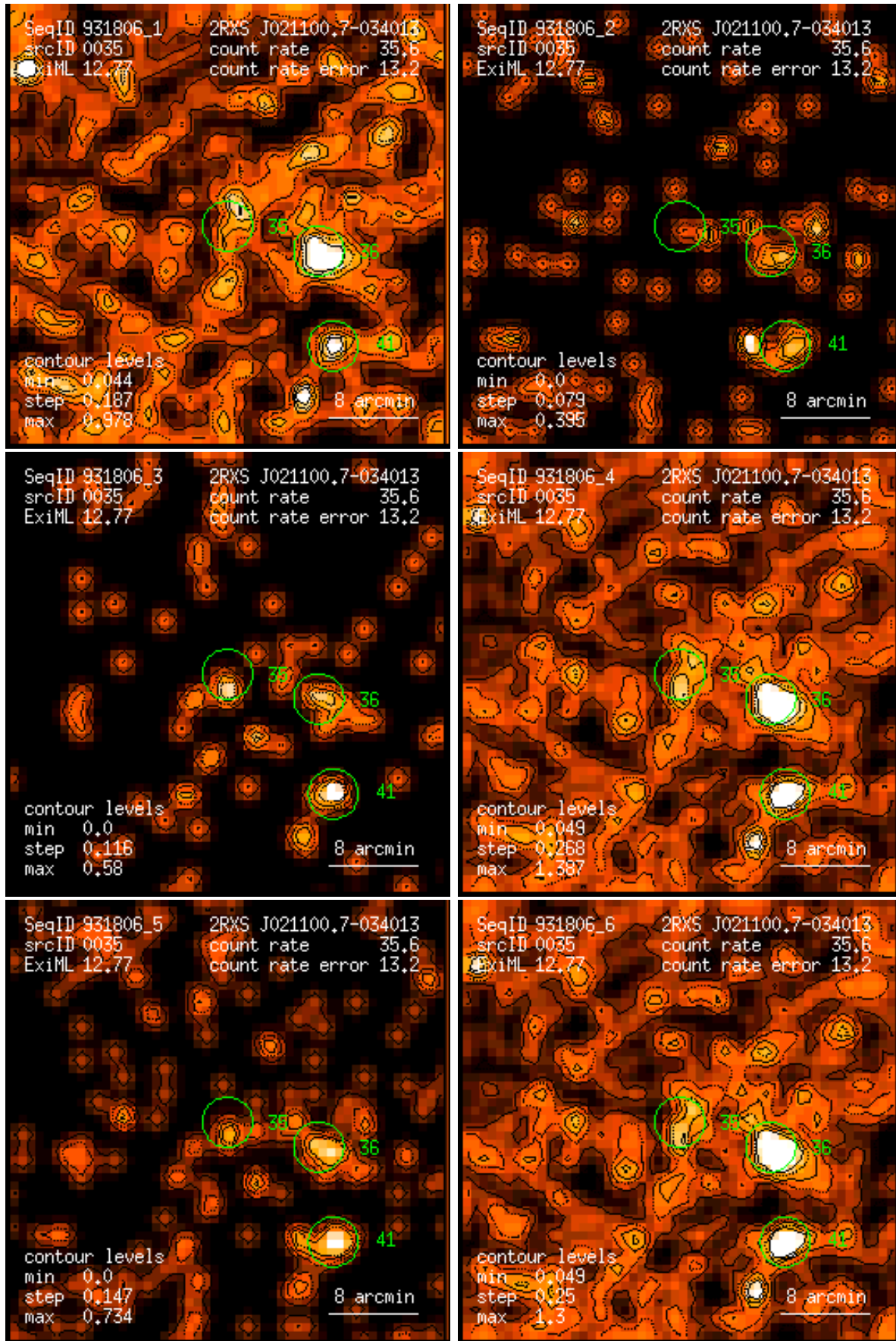
Figure 35: RASS 931806: detection 0035: band rate images, Gaussian filter: (1) PSPC channels 11 – 41, (2) 52 – 90, (3) 91 – 201, (4) 11 – 235, (5) 52 – 201, (6) 11 – 201. Broad band rates in counts/ks. Band rate contour levels in counts/ks/arcmin 2 .
