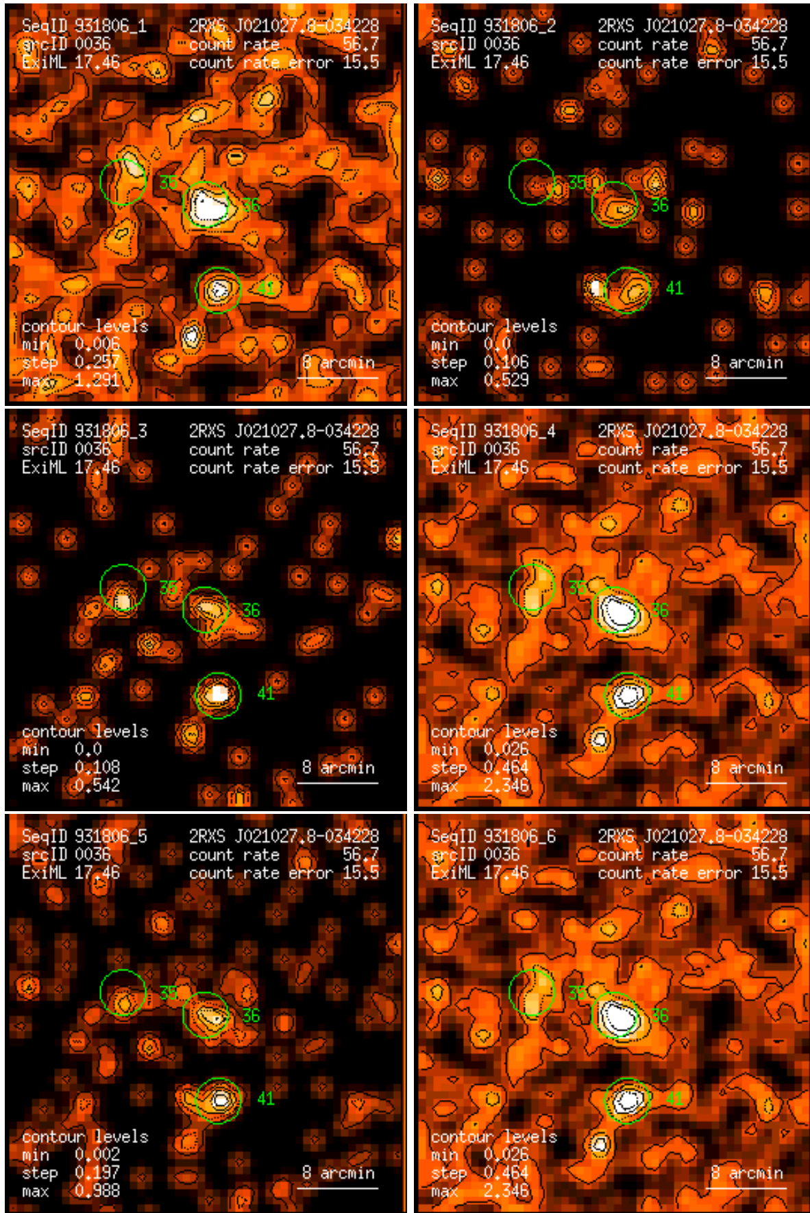
Figure 36: RASS 931806: detection 0036: band rate images, Gaussian filter: (1) PSPC channels 11 – 41, (2) 52 – 90, (3) 91 – 201, (4) 11 – 235, (5) 52 – 201, (6) 11 – 201. Broad band rates in counts/ks. Band rate contour levels in counts/ks/arcmin 2 .
