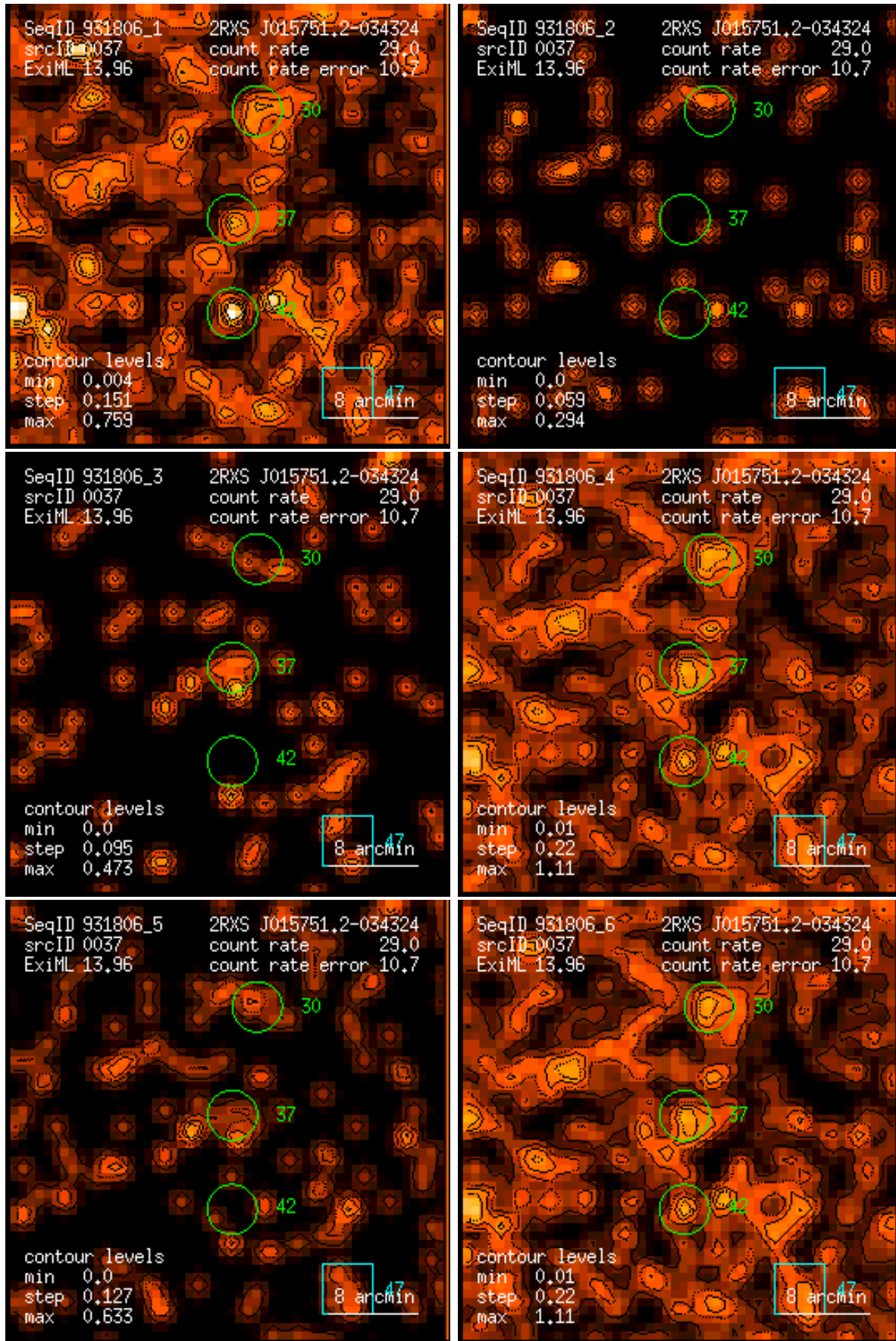
Figure 37: RASS 931806: detection 0037: band rate images, Gaussian filter: (1) PSPC channels 11 – 41, (2) 52 – 90, (3) 91 – 201, (4) 11 – 235, (5) 52 – 201, (6) 11 – 201. Broad band rates in counts/ks. Band rate contour levels in counts/ks/arcmin 2 .
