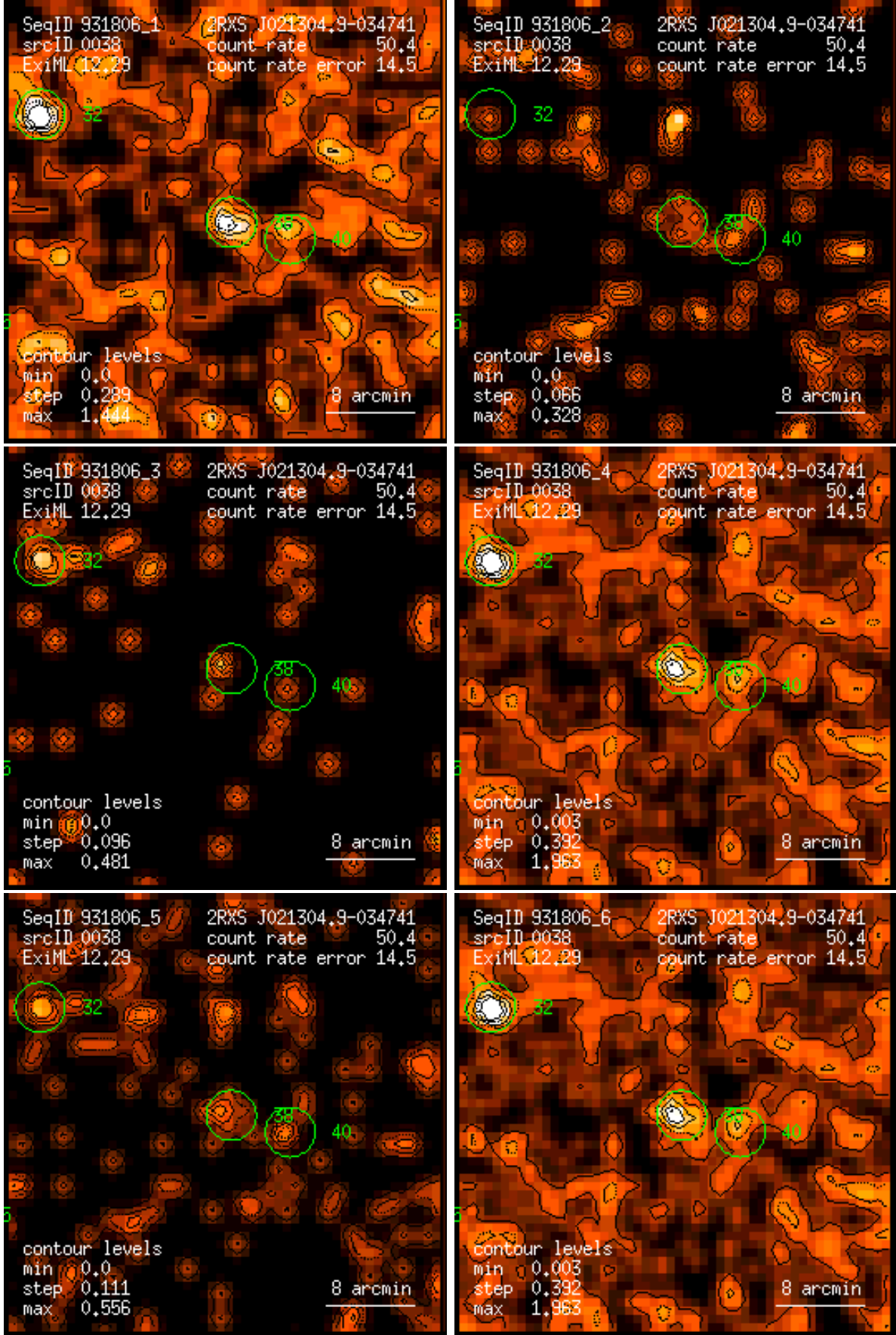
Figure 38: RASS 931806: detection 0038: band rate images, Gaussian filter: (1) PSPC channels 11 – 41, (2) 52 – 90, (3) 91 – 201, (4) 11 – 235, (5) 52 – 201, (6) 11 – 201. Broad band rates in counts/ks. Band rate contour levels in counts/ks/arcmin 2 .
