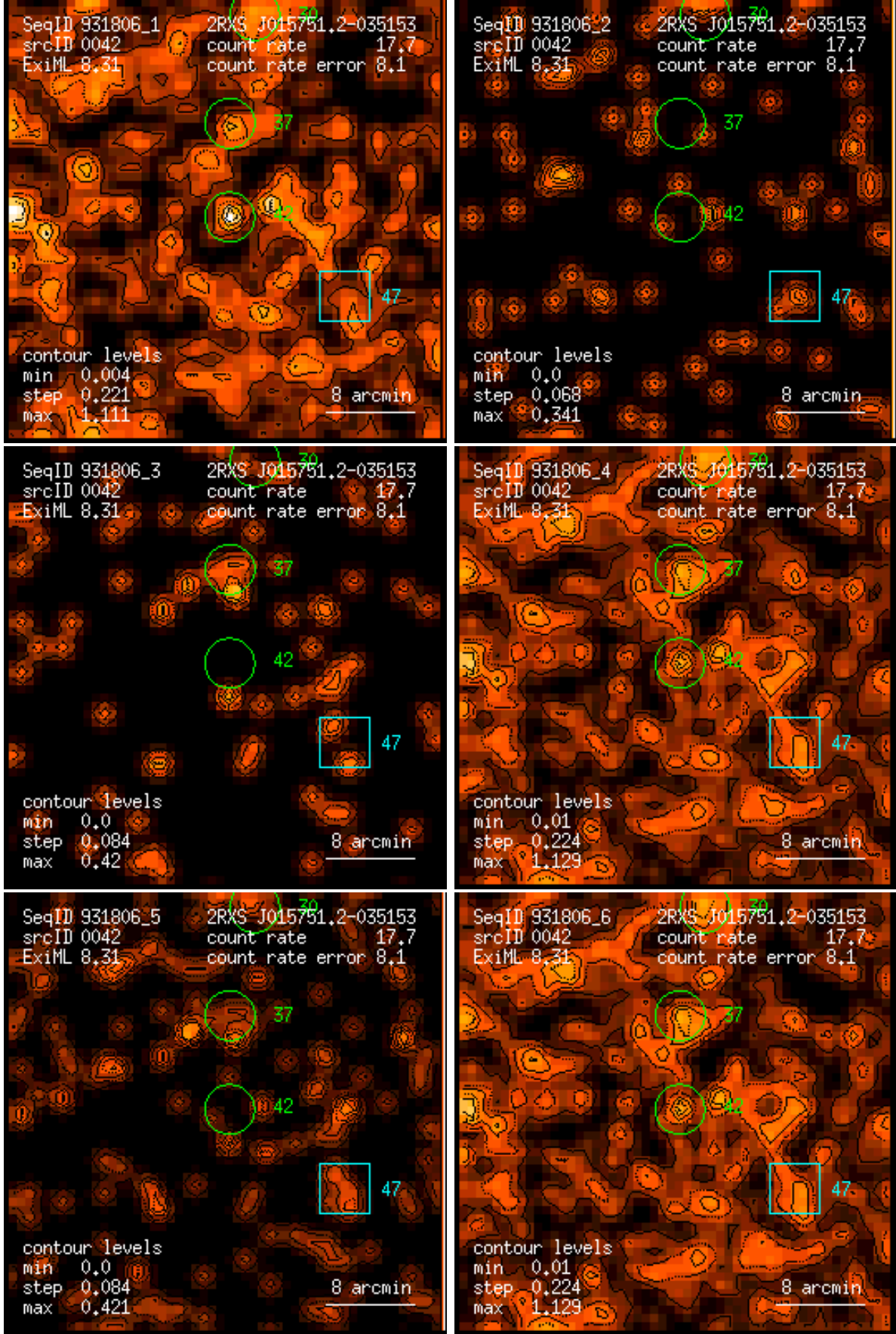
Figure 42: RASS 931806: detection 0042: band rate images, Gaussian filter: (1) PSPC channels 11 – 41, (2) 52 – 90, (3) 91 – 201, (4) 11 – 235, (5) 52 – 201, (6) 11 – 201. Broad band rates in counts/ks. Band rate contour levels in counts/ks/arcmin 2 .
