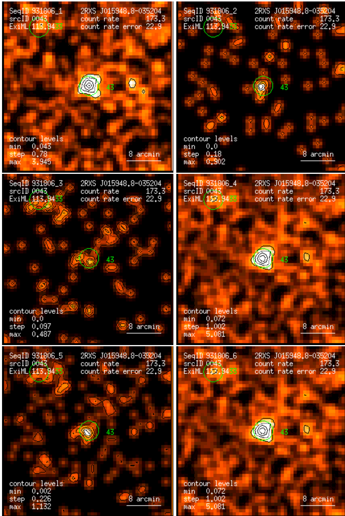
Figure 43: RASS 931806: detection 0043: band rate images, Gaussian filter: (1) PSPC channels 11 – 41, (2) 52 – 90, (3) 91 – 201, (4) 11 – 235, (5) 52 – 201, (6) 11 – 201. Broad band rates in counts/ks. Band rate contour levels in counts/ks/arcmin 2 .
