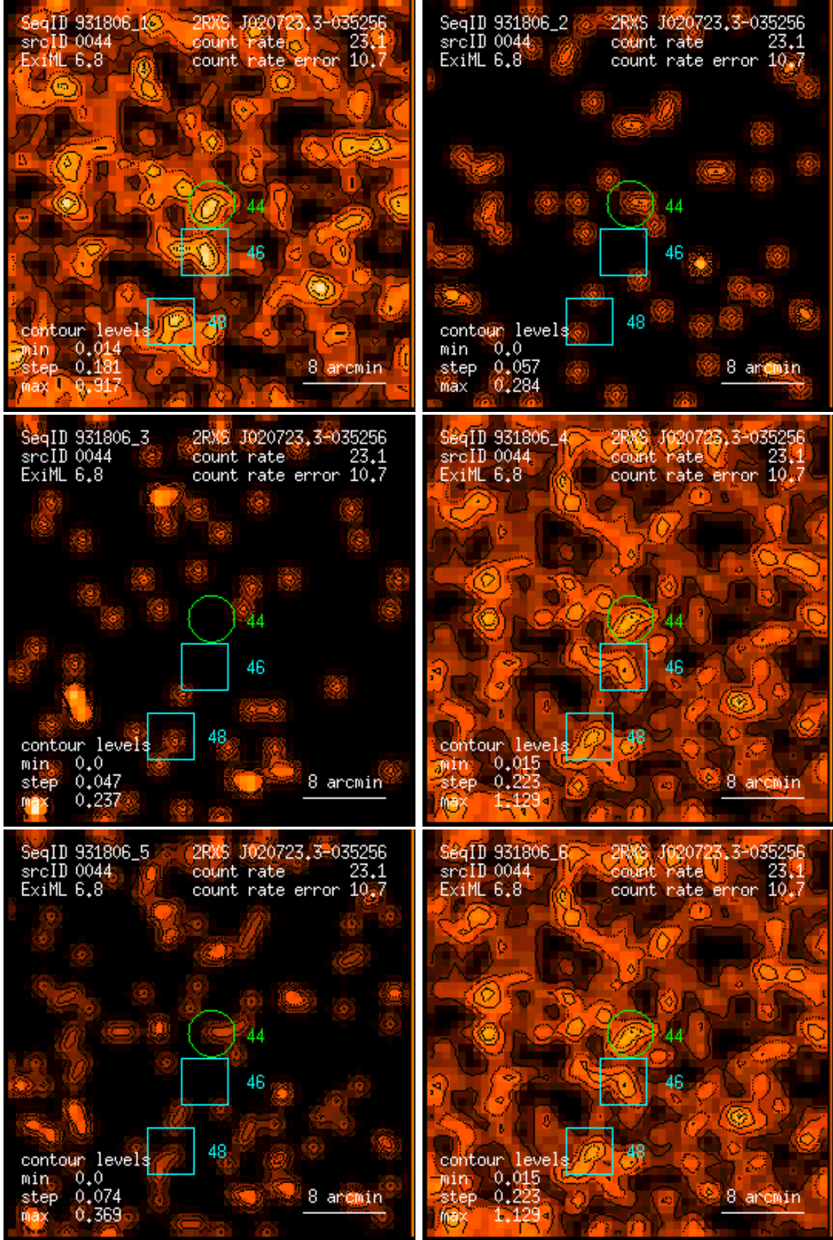
Figure 44: RASS 931806: detection 0044: band rate images, Gaussian filter: (1) PSPC channels 11 – 41, (2) 52 – 90, (3) 91 – 201, (4) 11 – 235, (5) 52 – 201, (6) 11 – 201. Broad band rates in counts/ks. Band rate contour levels in counts/ks/arcmin 2 .
