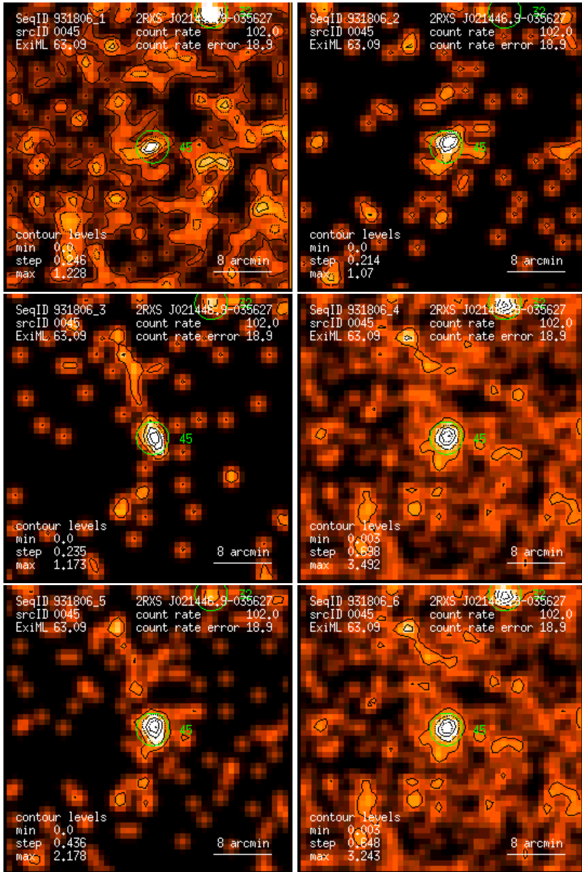
Figure 45: RASS 931806: detection 0045: band rate images, Gaussian filter: (1) PSPC channels 11 – 41, (2) 52 – 90, (3) 91 – 201, (4) 11 – 235, (5) 52 – 201, (6) 11 – 201. Broad band rates in counts/ks. Band rate contour levels in counts/ks/arcmin 2 .
