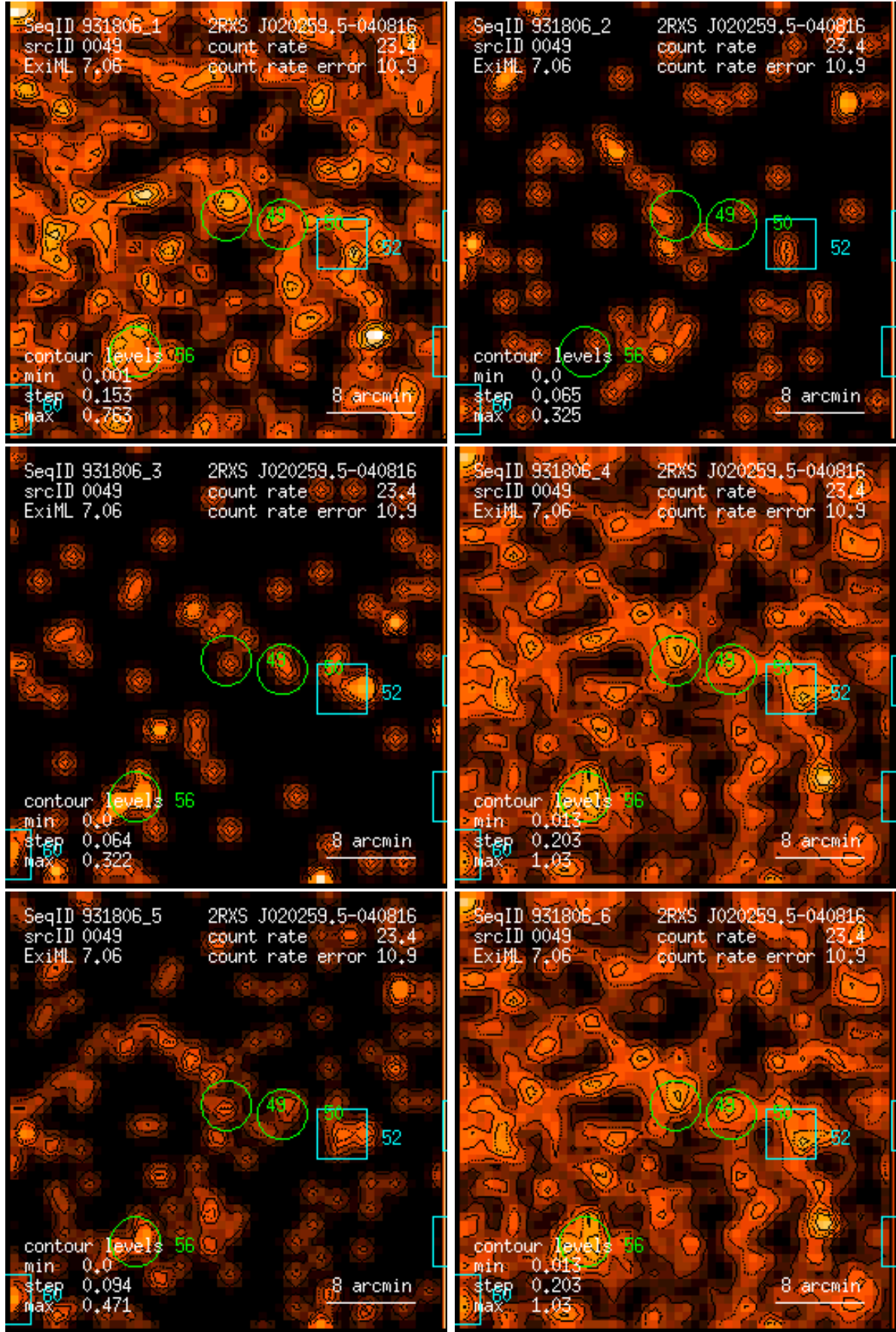
Figure 49: RASS 931806: detection 0049: band rate images, Gaussian filter: (1) PSPC channels 11 – 41, (2) 52 – 90, (3) 91 – 201, (4) 11 – 235, (5) 52 – 201, (6) 11 – 201. Broad band rates in counts/ks. Band rate contour levels in counts/ks/arcmin 2 .
