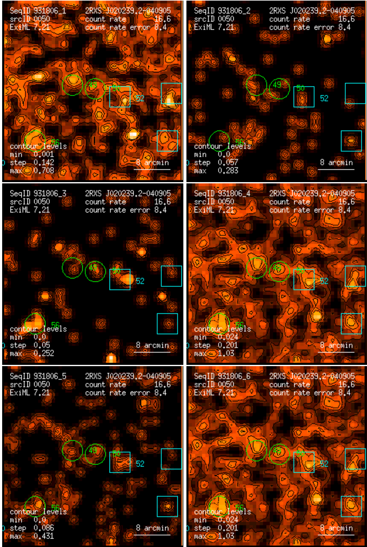
Figure 50: RASS 931806: detection 0050: band rate images, Gaussian filter: (1) PSPC channels 11 – 41, (2) 52 – 90, (3) 91 – 201, (4) 11 – 235, (5) 52 – 201, (6) 11 – 201. Broad band rates in counts/ks. Band rate contour levels in counts/ks/arcmin 2 .
