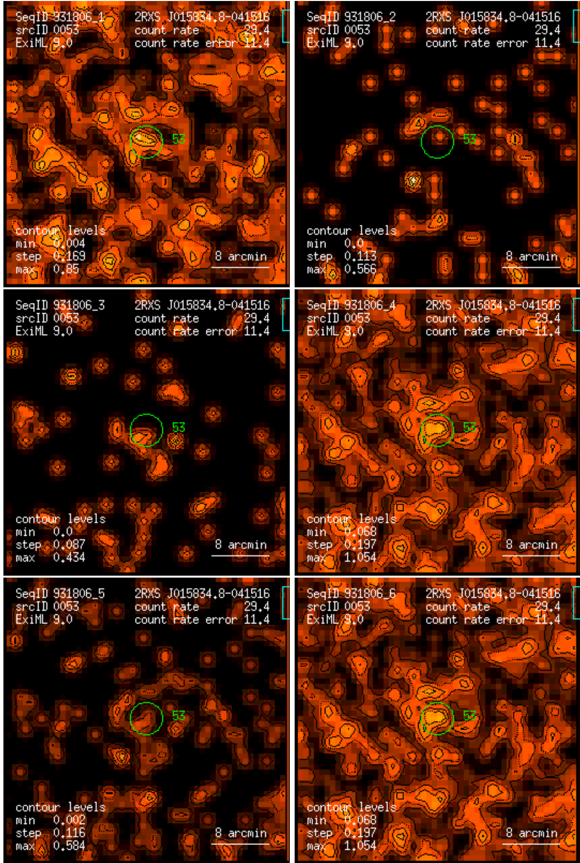
Figure 53: RASS 931806: detection 0053: band rate images, Gaussian filter: (1) PSPC channels 11 – 41, (2) 52 – 90, (3) 91 – 201, (4) 11 – 235, (5) 52 – 201, (6) 11 – 201. Broad band rates in counts/ks. Band rate contour levels in counts/ks/arcmin 2 .
