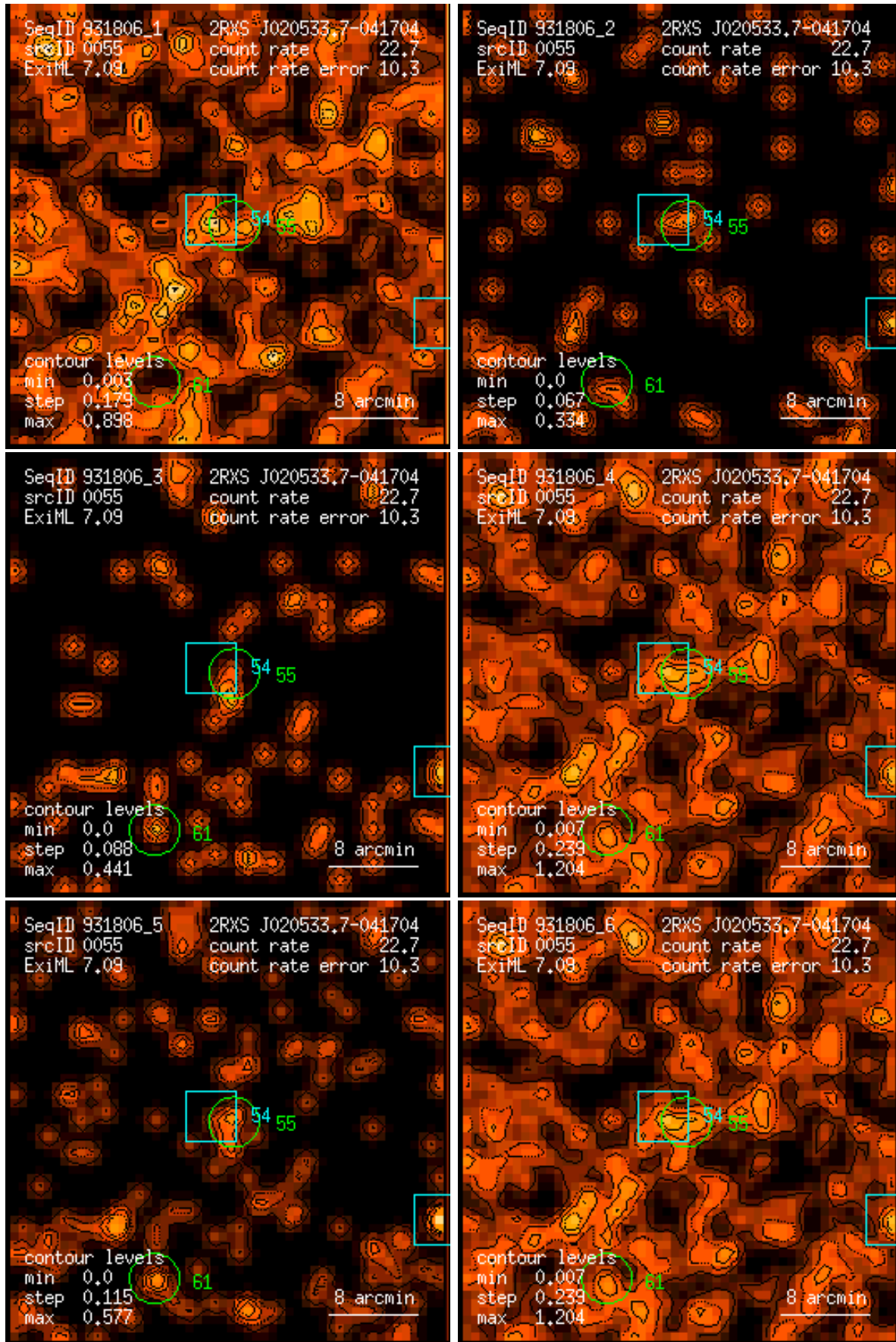
Figure 55: RASS 931806: detection 0055: band rate images, Gaussian filter: (1) PSPC channels 11 – 41, (2) 52 – 90, (3) 91 – 201, (4) 11 – 235, (5) 52 – 201, (6) 11 – 201. Broad band rates in counts/ks. Band rate contour levels in counts/ks/arcmin 2 .
