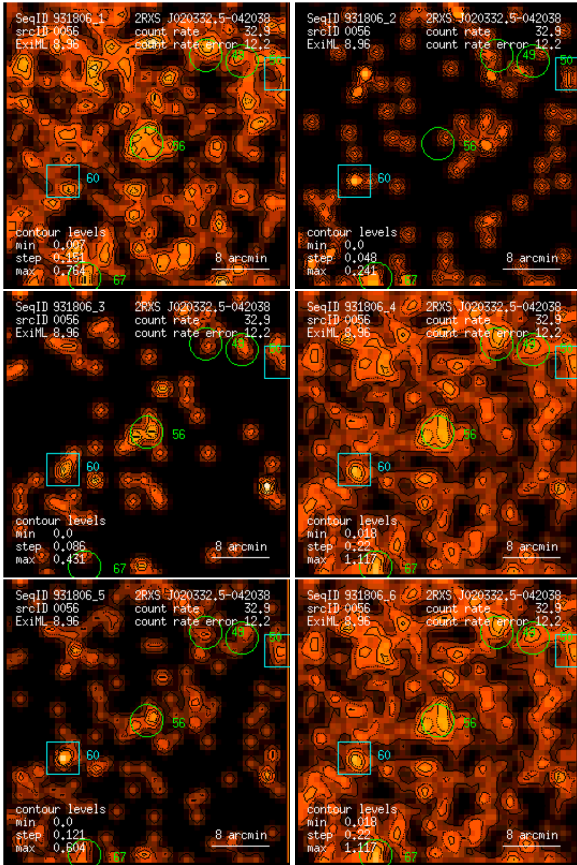
Figure 56: RASS 931806: detection 0056: band rate images, Gaussian filter: (1) PSPC channels 11 – 41, (2) 52 – 90, (3) 91 – 201, (4) 11 – 235, (5) 52 – 201, (6) 11 – 201. Broad band rates in counts/ks. Band rate contour levels in counts/ks/arcmin 2 .
