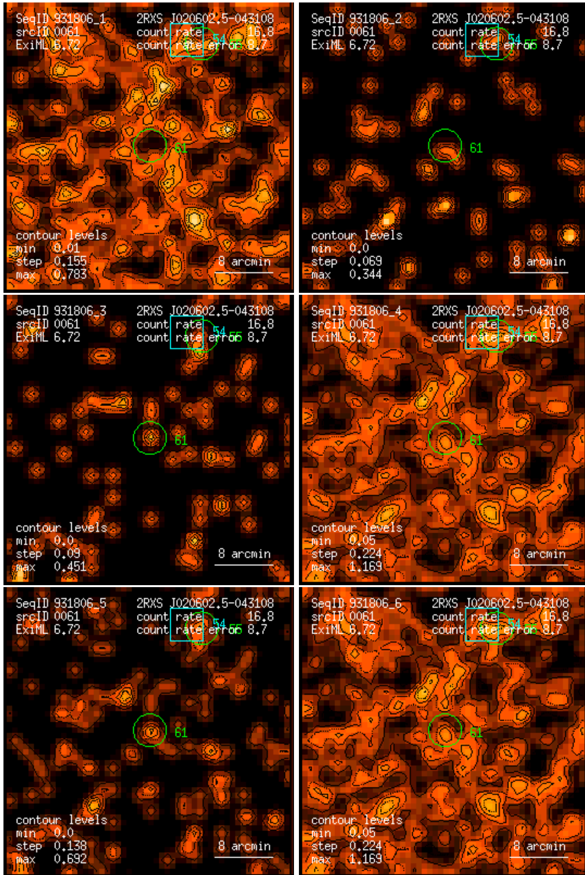
Figure 61: RASS 931806: detection 0061: band rate images, Gaussian filter: (1) PSPC channels 11 – 41, (2) 52 – 90, (3) 91 – 201, (4) 11 – 235, (5) 52 – 201, (6) 11 – 201. Broad band rates in counts/ks. Band rate contour levels in counts/ks/arcmin 2 .
