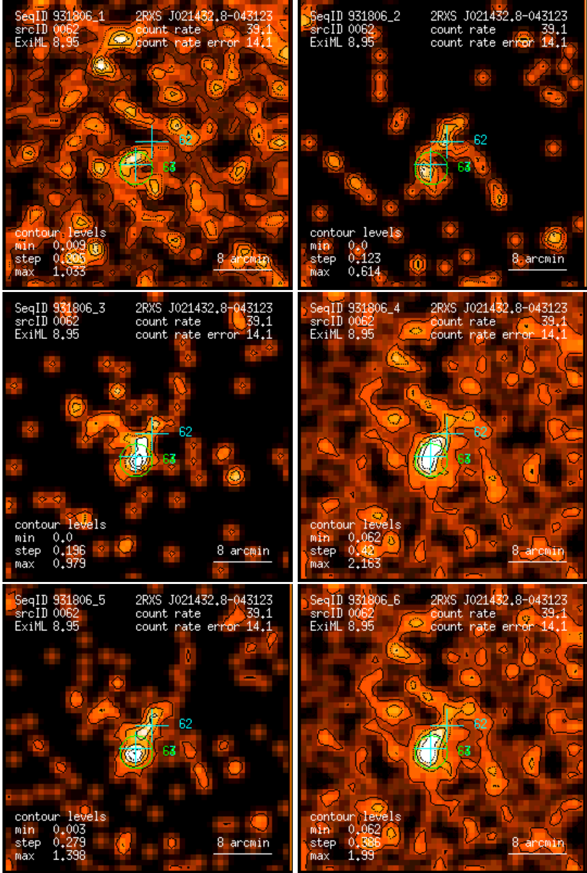
Figure 62: RASS 931806: detection 0062: band rate images, Gaussian filter: (1) PSPC channels 11 – 41, (2) 52 – 90, (3) 91 – 201, (4) 11 – 235, (5) 52 – 201, (6) 11 – 201. Broad band rates in counts/ks. Band rate contour levels in counts/ks/arcmin 2 .
