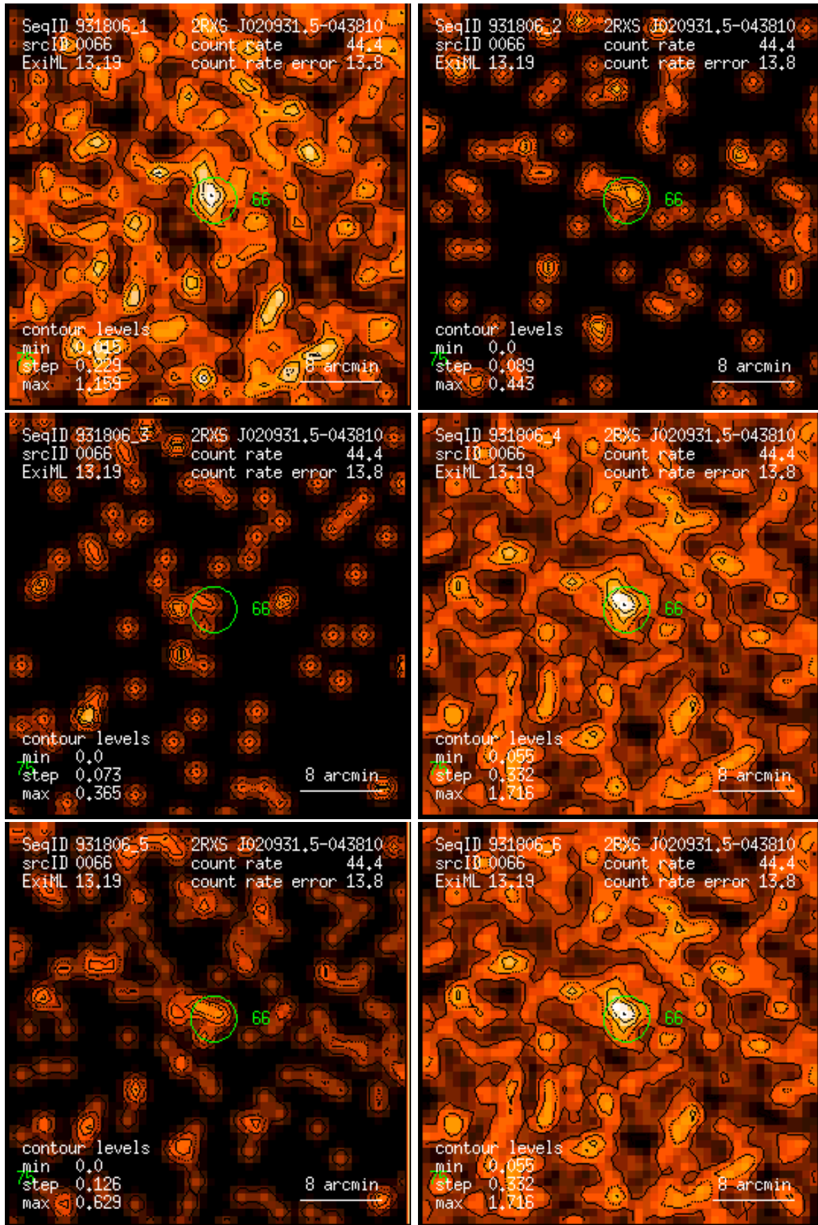
Figure 66: RASS 931806: detection 0066: band rate images, Gaussian filter: (1) PSPC channels 11 – 41, (2) 52 – 90, (3) 91 – 201, (4) 11 – 235, (5) 52 – 201, (6) 11 – 201. Broad band rates in counts/ks. Band rate contour levels in counts/ks/arcmin 2 .
