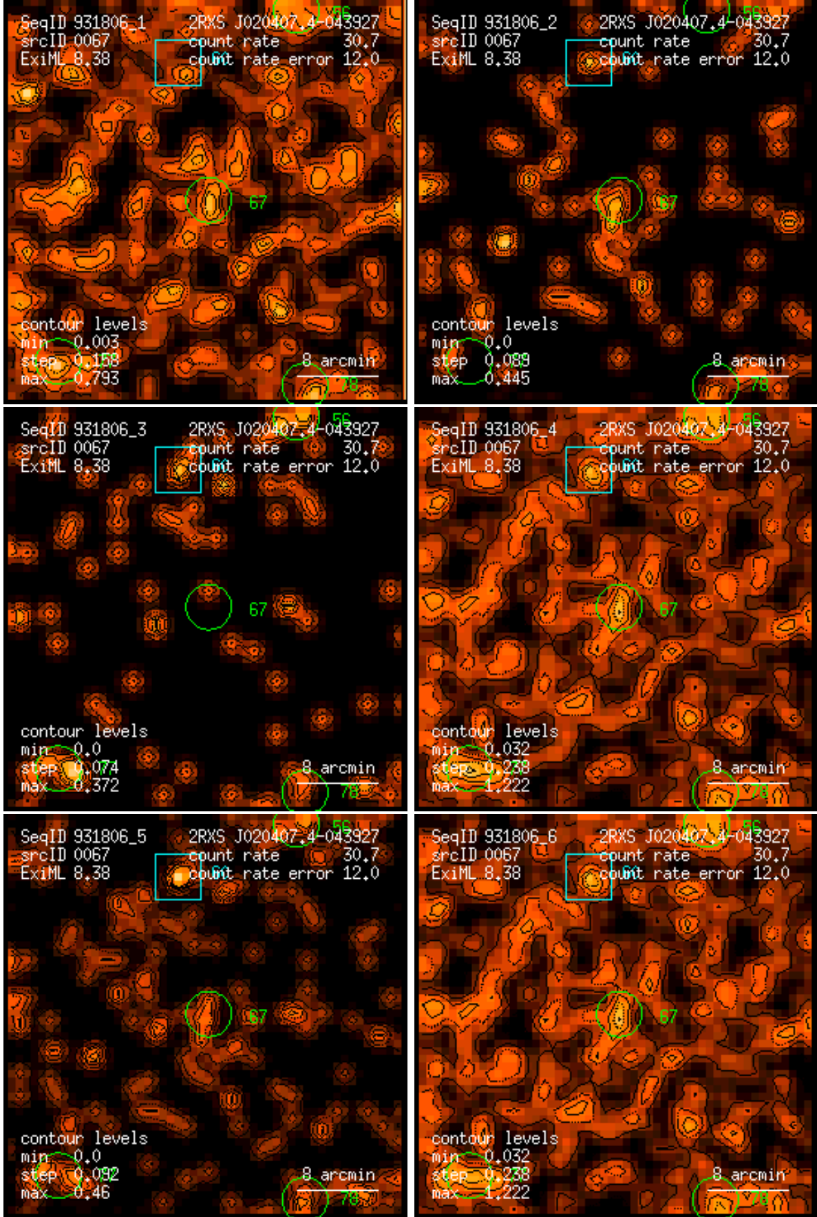
Figure 67: RASS 931806: detection 0067: band rate images, Gaussian filter: (1) PSPC channels 11 – 41, (2) 52 – 90, (3) 91 – 201, (4) 11 – 235, (5) 52 – 201, (6) 11 – 201. Broad band rates in counts/ks. Band rate contour levels in counts/ks/arcmin 2 .
