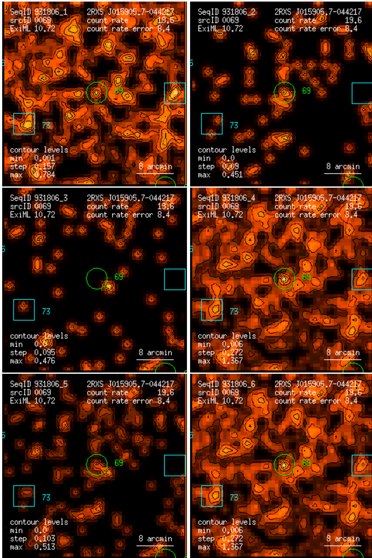
Figure 69: RASS 931806: detection 0069: band rate images, Gaussian filter: (1) PSPC channels 11 – 41, (2) 52 – 90, (3) 91 – 201, (4) 11 – 235, (5) 52 – 201, (6) 11 – 201. Broad band rates in counts/ks. Band rate contour levels in counts/ks/arcmin 2 .
