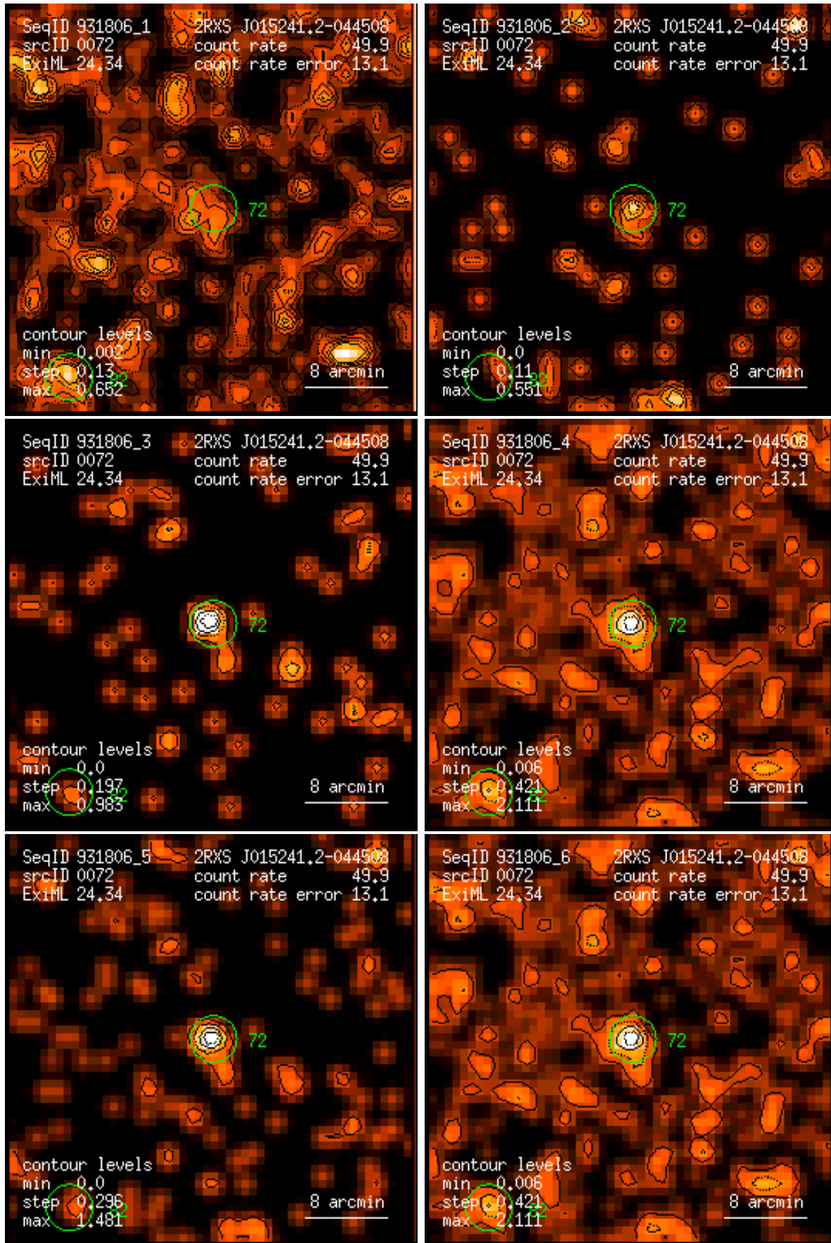
Figure 72: RASS 931806: detection 0072: band rate images, Gaussian filter: (1) PSPC channels 11 – 41, (2) 52 – 90, (3) 91 – 201, (4) 11 – 235, (5) 52 – 201, (6) 11 – 201. Broad band rates in counts/ks. Band rate contour levels in counts/ks/arcmin 2 .
