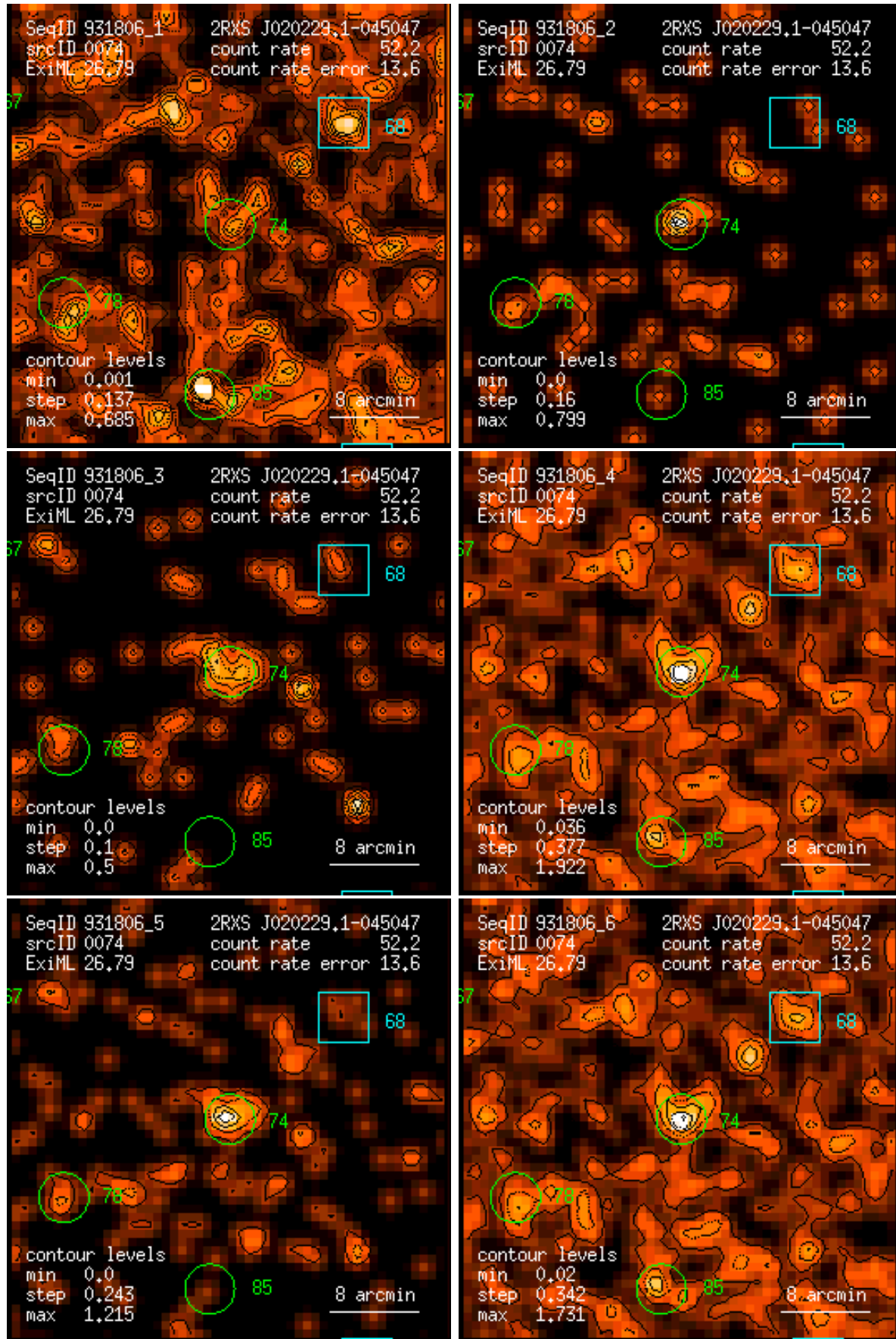
Figure 74: RASS 931806: detection 0074: band rate images, Gaussian filter: (1) PSPC channels 11 – 41, (2) 52 – 90, (3) 91 – 201, (4) 11 – 235, (5) 52 – 201, (6) 11 – 201. Broad band rates in counts/ks. Band rate contour levels in counts/ks/arcmin 2 .
