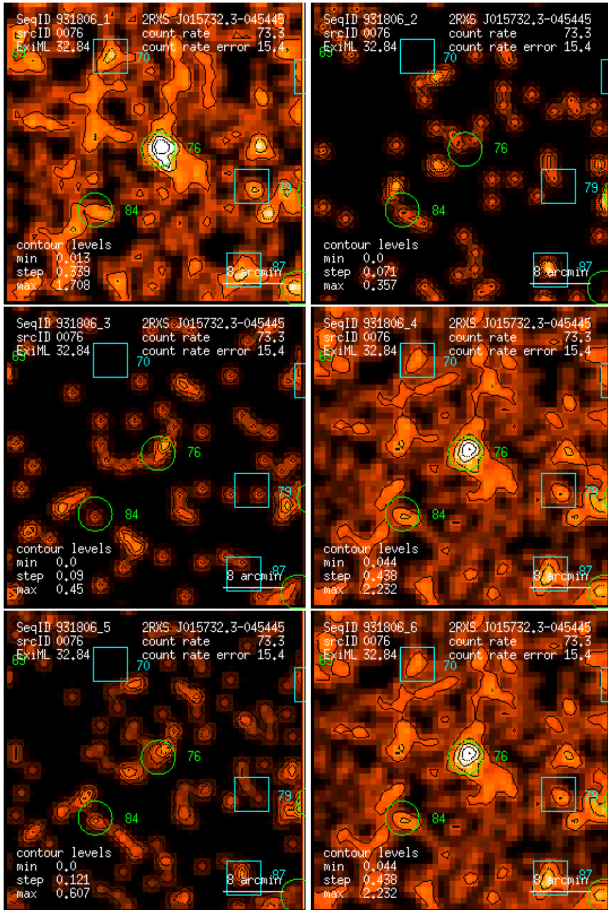
Figure 76: RASS 931806: detection 0076: band rate images, Gaussian filter: (1) PSPC channels 11 – 41, (2) 52 – 90, (3) 91 – 201, (4) 11 – 235, (5) 52 – 201, (6) 11 – 201. Broad band rates in counts/ks. Band rate contour levels in counts/ks/arcmin 2 .
