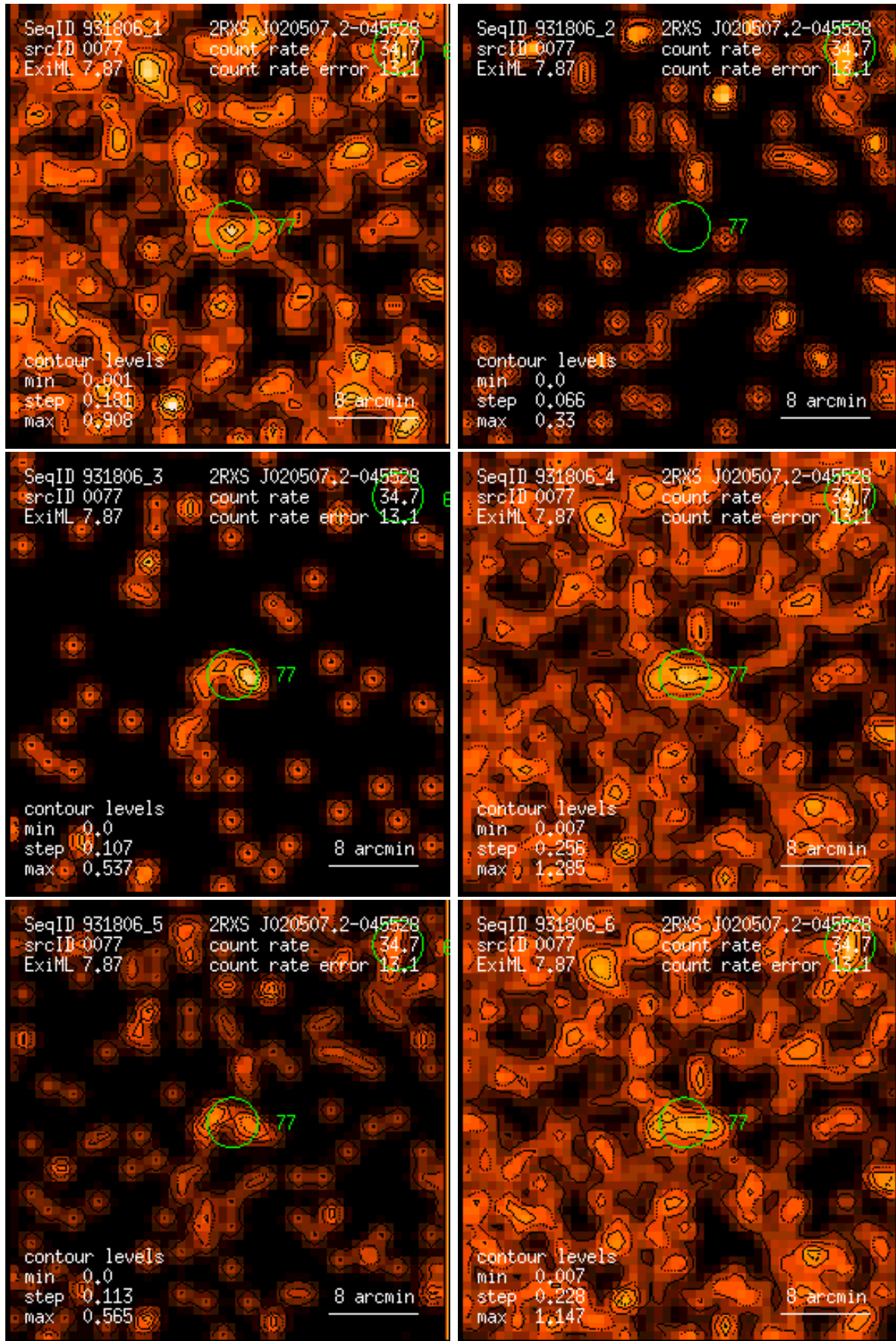
Figure 77: RASS 931806: detection 0077: band rate images, Gaussian filter: (1) PSPC channels 11 – 41, (2) 52 – 90, (3) 91 – 201, (4) 11 – 235, (5) 52 – 201, (6) 11 – 201. Broad band rates in counts/ks. Band rate contour levels in counts/ks/arcmin 2 .
