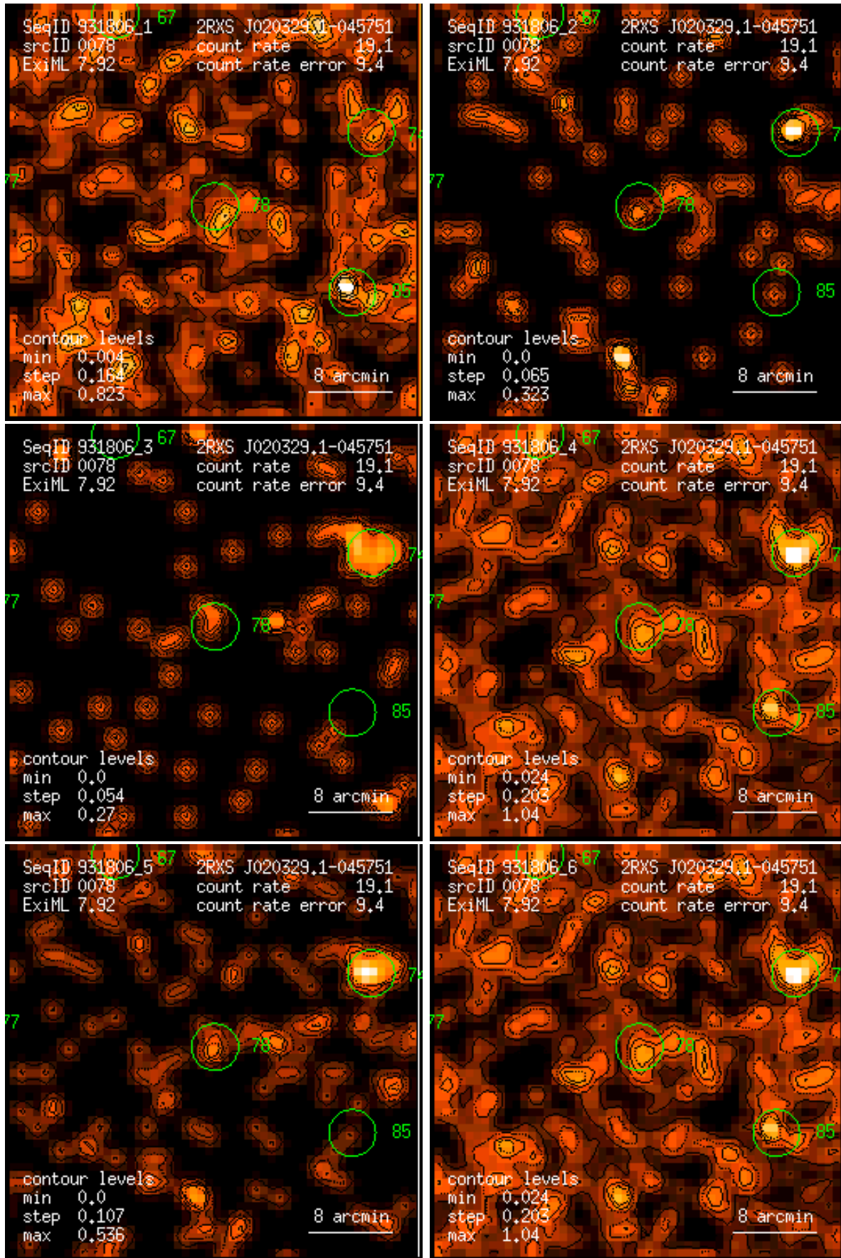
Figure 78: RASS 931806: detection 0078: band rate images, Gaussian filter: (1) PSPC channels 11 – 41, (2) 52 – 90, (3) 91 – 201, (4) 11 – 235, (5) 52 – 201, (6) 11 – 201. Broad band rates in counts/ks. Band rate contour levels in counts/ks/arcmin 2 .
