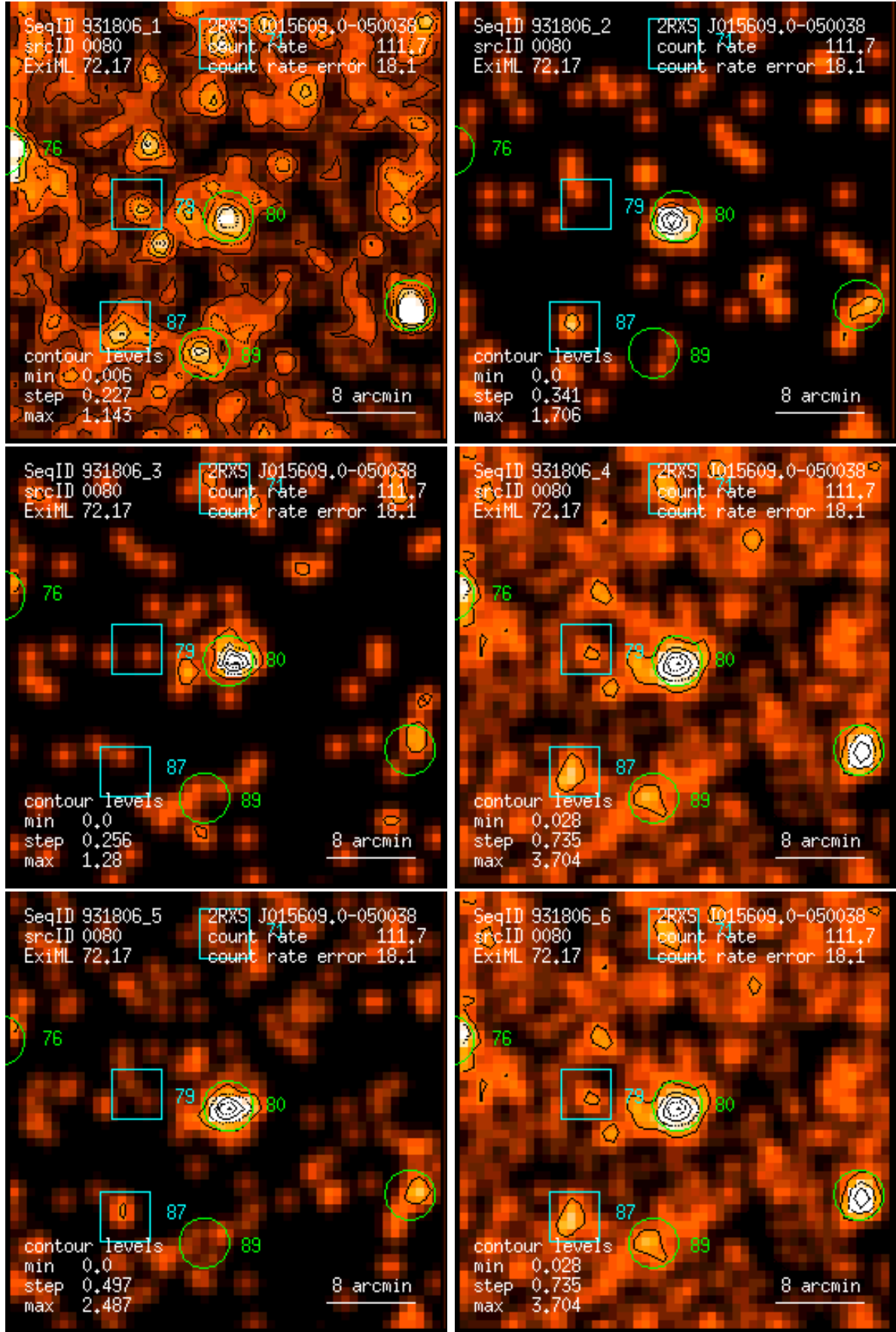
Figure 80: RASS 931806: detection 0080: band rate images, Gaussian filter: (1) PSPC channels 11 – 41, (2) 52 – 90, (3) 91 – 201, (4) 11 – 235, (5) 52 – 201, (6) 11 – 201. Broad band rates in counts/ks. Band rate contour levels in counts/ks/arcmin 2 .
