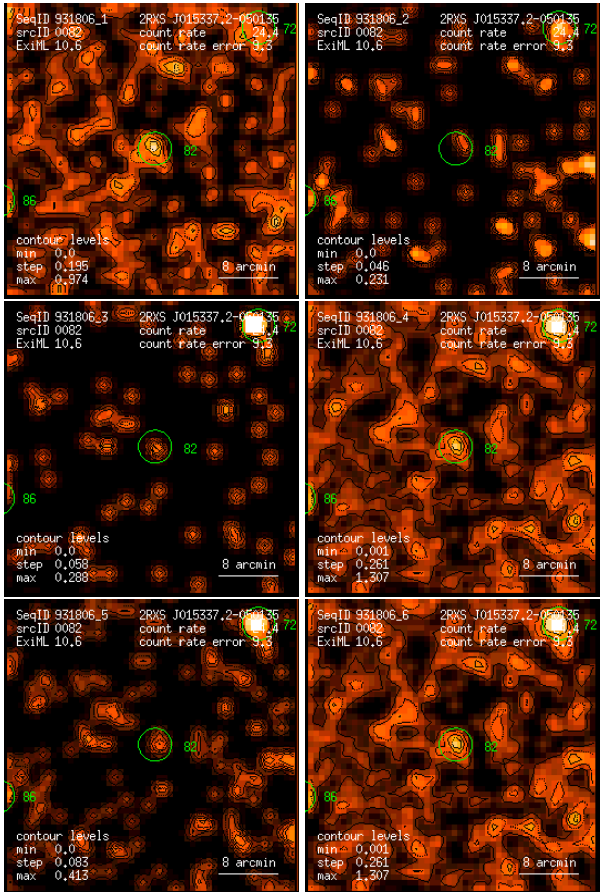
Figure 82: RASS 931806: detection 0082: band rate images, Gaussian filter: (1) PSPC channels 11 – 41, (2) 52 – 90, (3) 91 – 201, (4) 11 – 235, (5) 52 – 201, (6) 11 – 201. Broad band rates in counts/ks. Band rate contour levels in counts/ks/arcmin 2 .
