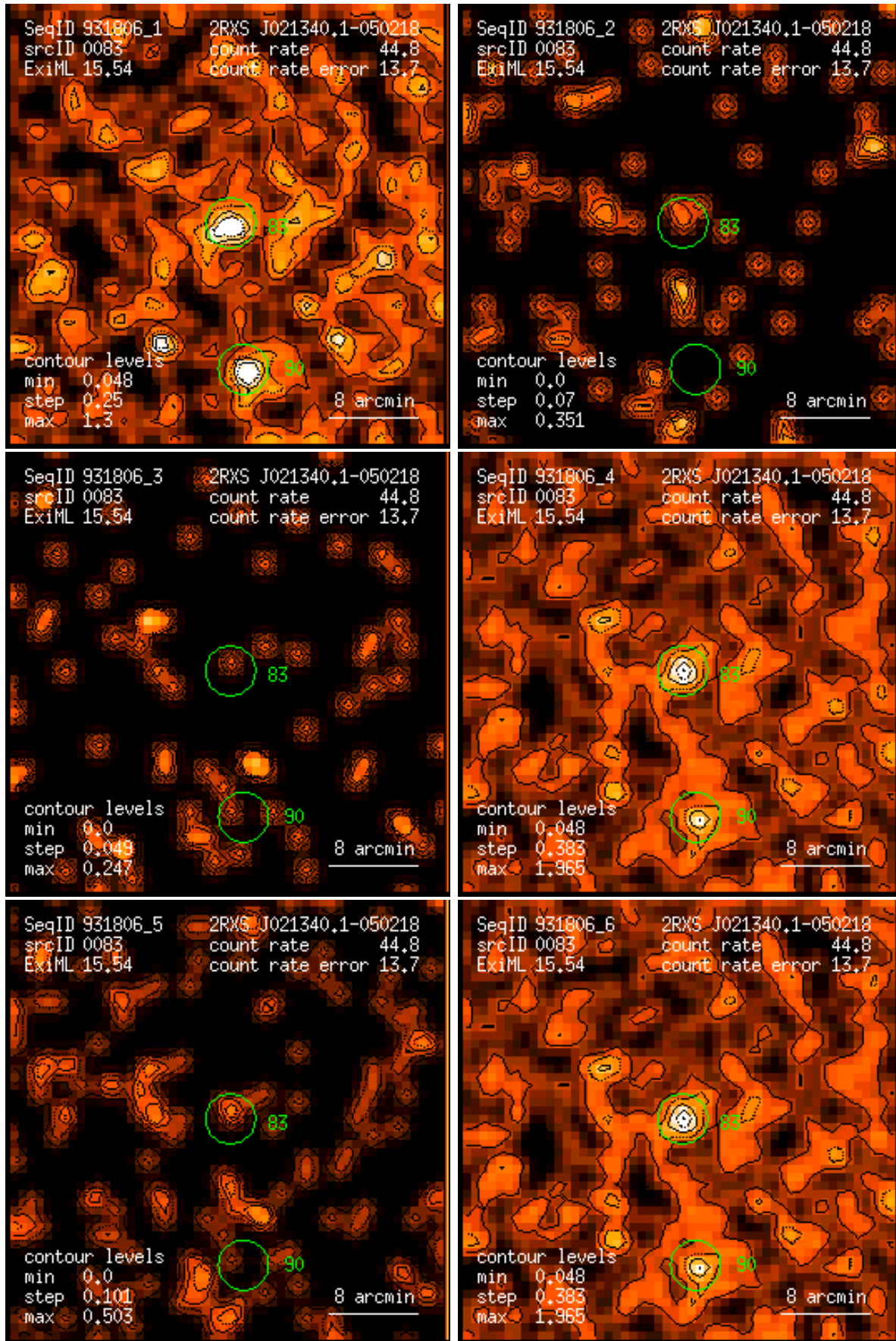
Figure 83: RASS 931806: detection 0083: band rate images, Gaussian filter: (1) PSPC channels 11 – 41, (2) 52 – 90, (3) 91 – 201, (4) 11 – 235, (5) 52 – 201, (6) 11 – 201. Broad band rates in counts/ks. Band rate contour levels in counts/ks/arcmin 2 .
