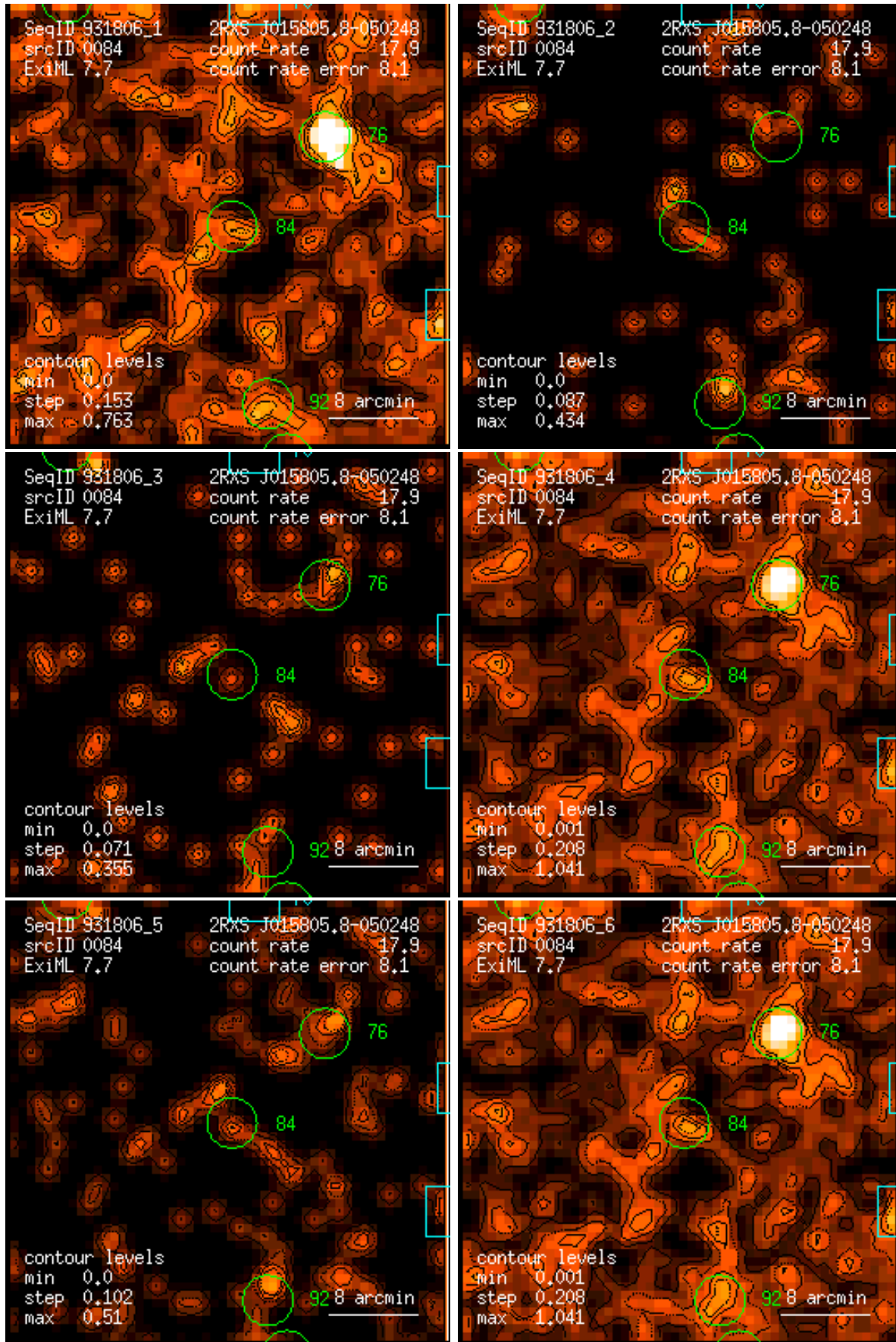
Figure 84: RASS 931806: detection 0084: band rate images, Gaussian filter: (1) PSPC channels 11 – 41, (2) 52 – 90, (3) 91 – 201, (4) 11 – 235, (5) 52 – 201, (6) 11 – 201. Broad band rates in counts/ks. Band rate contour levels in counts/ks/arcmin 2 .
