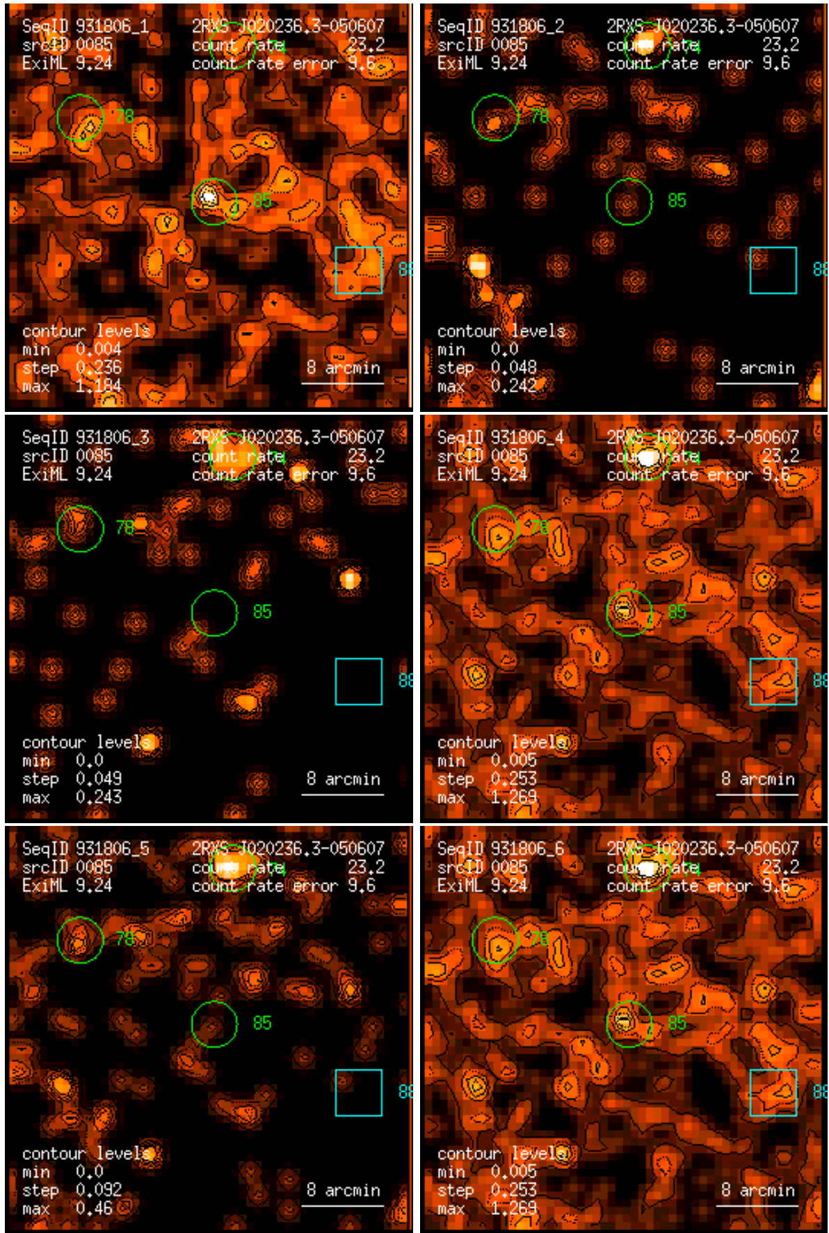
Figure 85: RASS 931806: detection 0085: band rate images, Gaussian filter: (1) PSPC channels 11 – 41, (2) 52 – 90, (3) 91 – 201, (4) 11 – 235, (5) 52 – 201, (6) 11 – 201. Broad band rates in counts/ks. Band rate contour levels in counts/ks/arcmin 2 .
