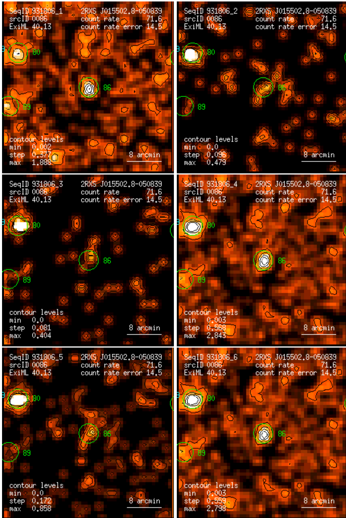
Figure 86: RASS 931806: detection 0086: band rate images, Gaussian filter: (1) PSPC channels 11 – 41, (2) 52 – 90, (3) 91 – 201, (4) 11 – 235, (5) 52 – 201, (6) 11 – 201. Broad band rates in counts/ks. Band rate contour levels in counts/ks/arcmin 2 .
