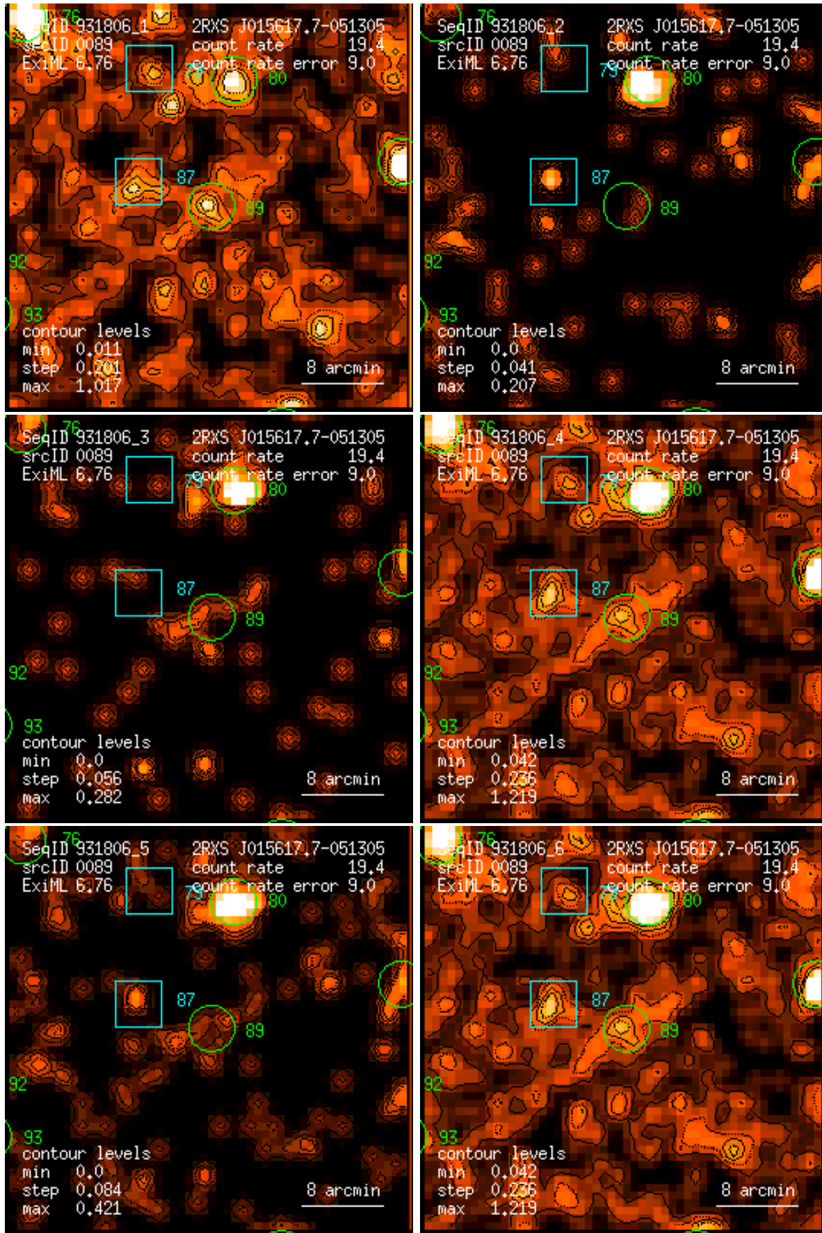
Figure 89: RASS 931806: detection 0089: band rate images, Gaussian filter: (1) PSPC channels 11 – 41, (2) 52 – 90, (3) 91 – 201, (4) 11 – 235, (5) 52 – 201, (6) 11 – 201. Broad band rates in counts/ks. Band rate contour levels in counts/ks/arcmin 2 .
