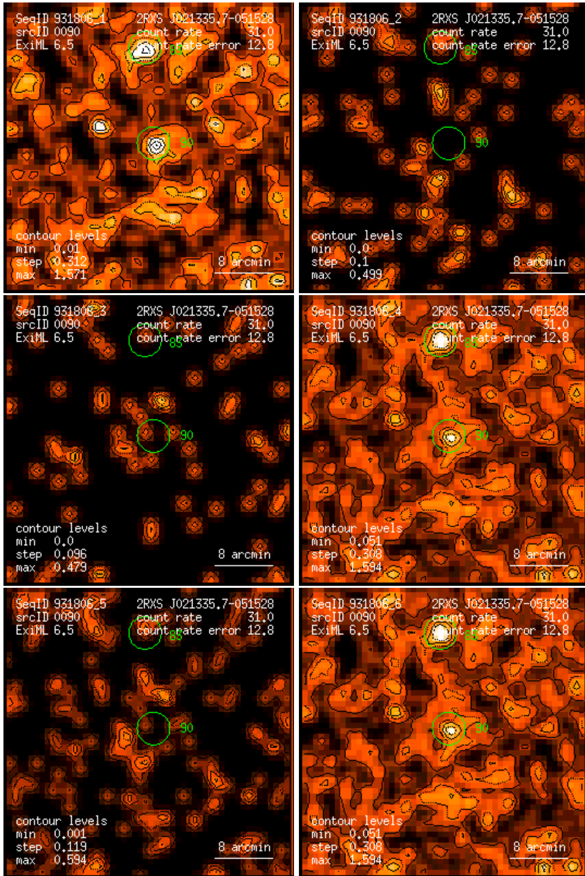
Figure 90: RASS 931806: detection 0090: band rate images, Gaussian filter: (1) PSPC channels 11 – 41, (2) 52 – 90, (3) 91 – 201, (4) 11 – 235, (5) 52 – 201, (6) 11 – 201. Broad band rates in counts/ks. Band rate contour levels in counts/ks/arcmin 2 .
