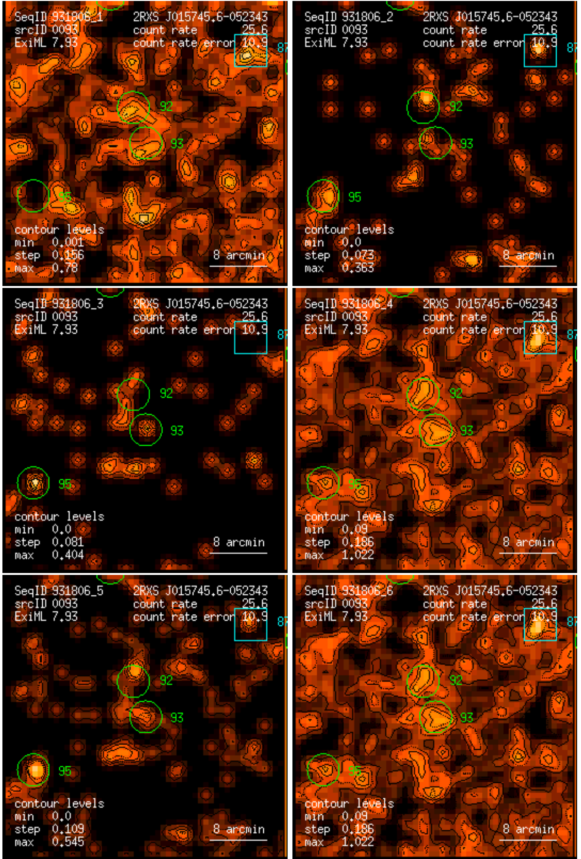
Figure 93: RASS 931806: detection 0093: band rate images, Gaussian filter: (1) PSPC channels 11 – 41, (2) 52 – 90, (3) 91 – 201, (4) 11 – 235, (5) 52 – 201, (6) 11 – 201. Broad band rates in counts/ks. Band rate contour levels in counts/ks/arcmin 2 .
