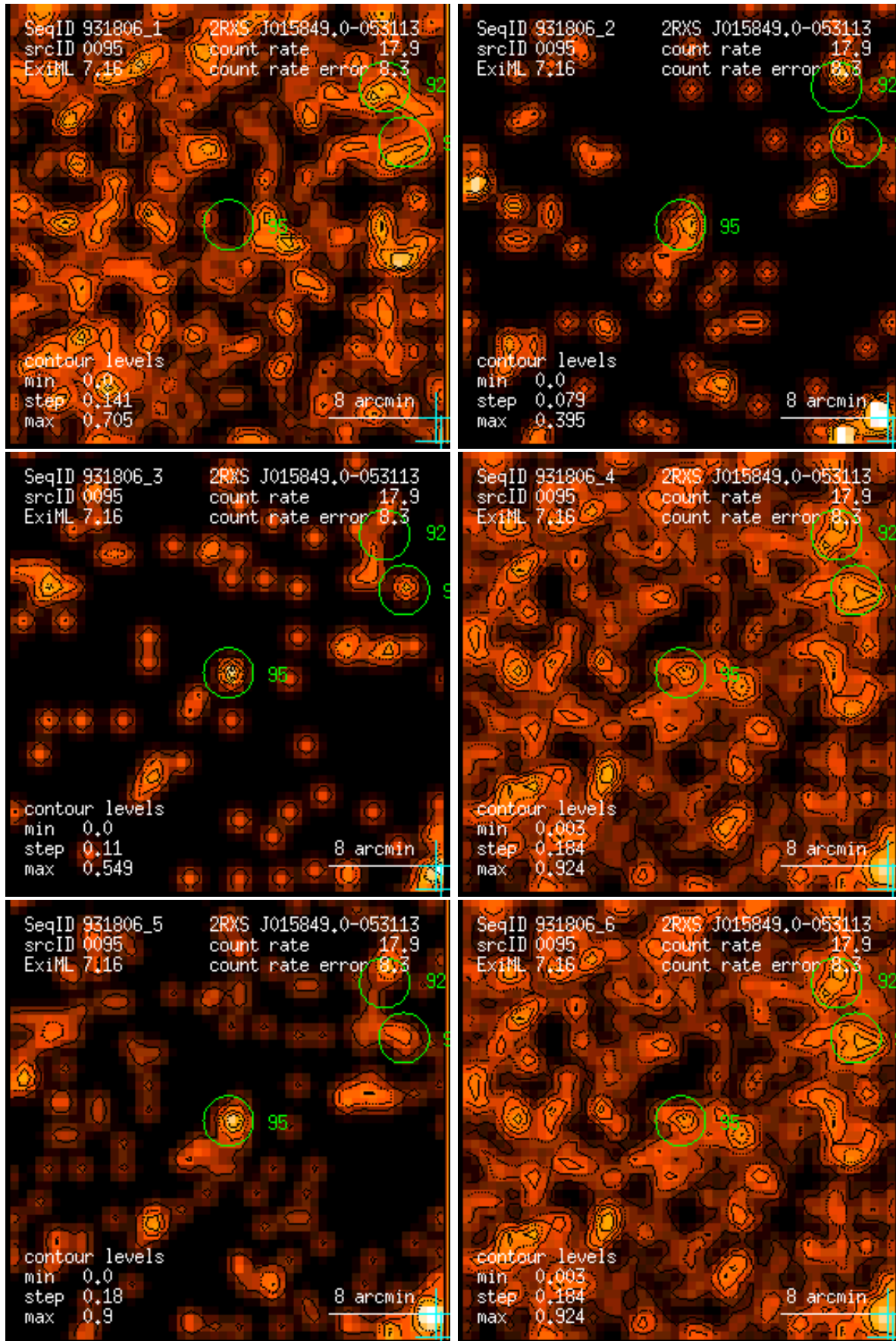
Figure 95: RASS 931806: detection 0095: band rate images, Gaussian filter: (1) PSPC channels 11 – 41, (2) 52 – 90, (3) 91 – 201, (4) 11 – 235, (5) 52 – 201, (6) 11 – 201. Broad band rates in counts/ks. Band rate contour levels in counts/ks/arcmin 2 .
