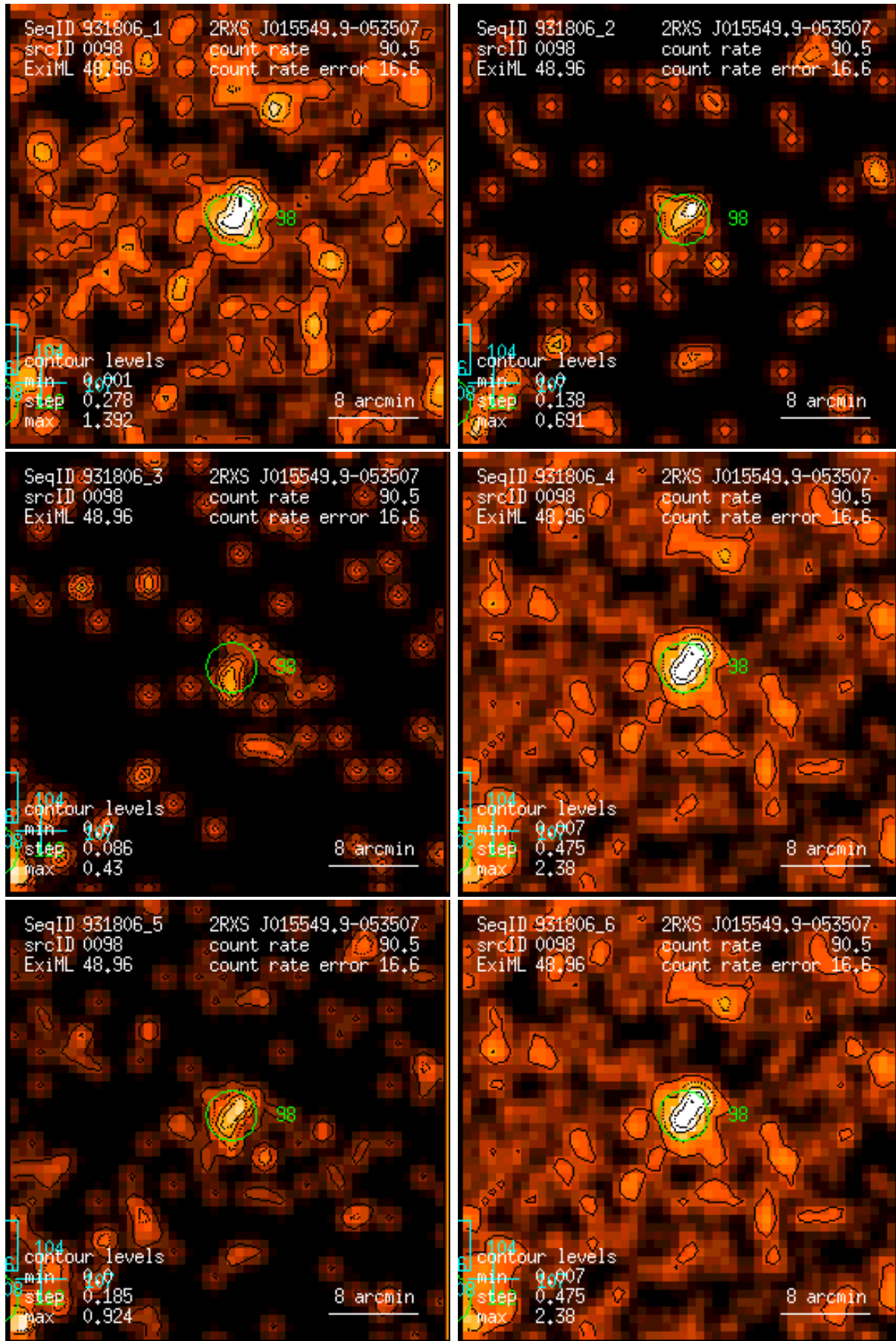
Figure 98: RASS 931806: detection 0098: band rate images, Gaussian filter: (1) PSPC channels 11 – 41, (2) 52 – 90, (3) 91 – 201, (4) 11 – 235, (5) 52 – 201, (6) 11 – 201. Broad band rates in counts/ks. Band rate contour levels in counts/ks/arcmin 2 .
