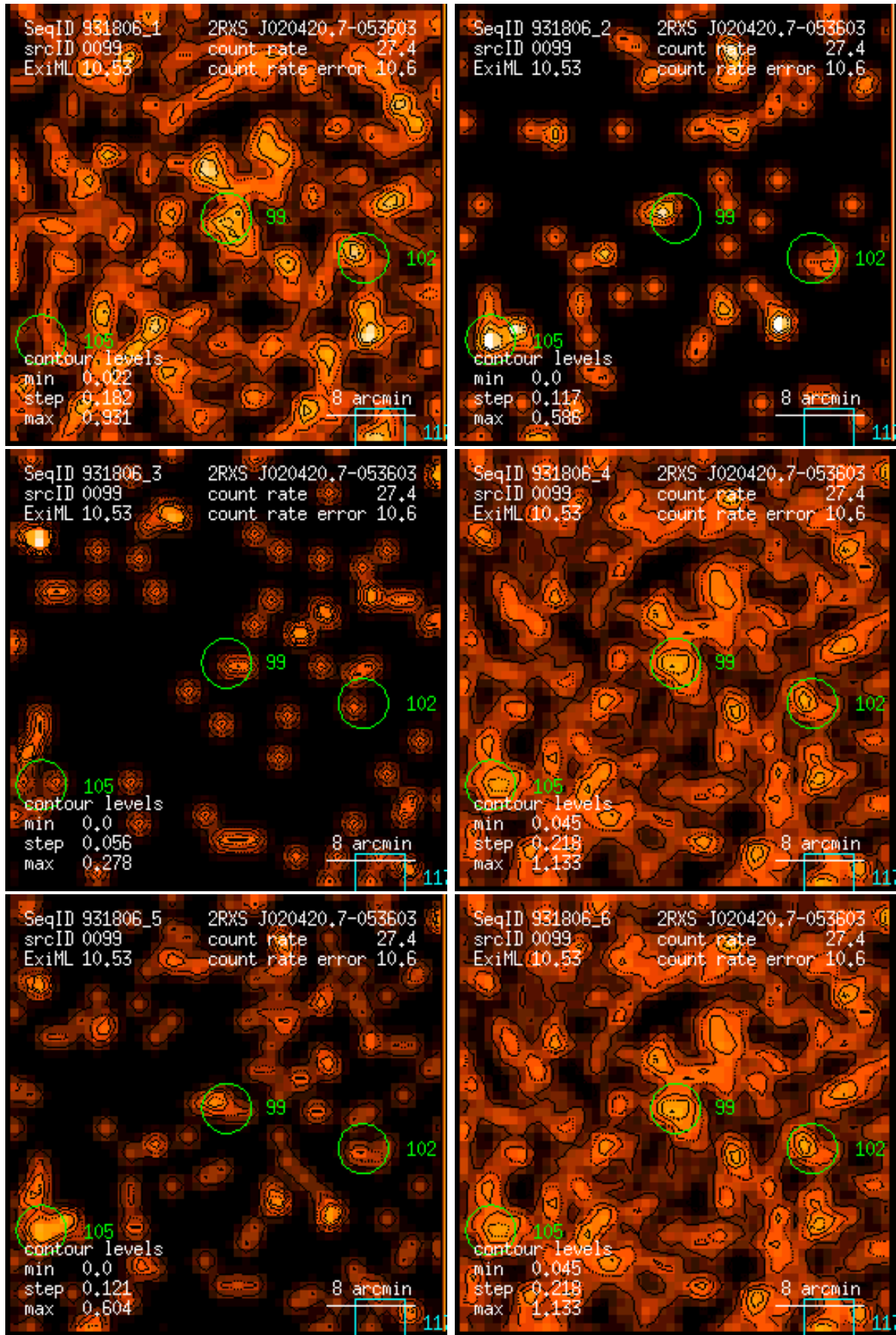
Figure 99: RASS 931806: detection 0099: band rate images, Gaussian filter: (1) PSPC channels 11 – 41, (2) 52 – 90, (3) 91 – 201, (4) 11 – 235, (5) 52 – 201, (6) 11 – 201. Broad band rates in counts/ks. Band rate contour levels in counts/ks/arcmin 2 .
