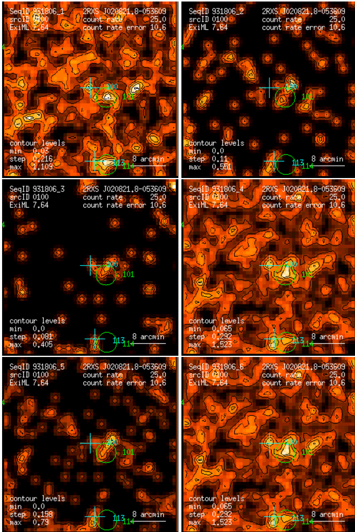
Figure 100: RASS 931806: detection 0100: band rate images, Gaussian filter: (1) PSPC channels 11 – 41, (2) 52 – 90, (3) 91 – 201, (4) 11 – 235, (5) 52 – 201, (6) 11 – 201. Broad band rates in counts/ks. Band rate contour levels in counts/ks/arcmin 2 .
