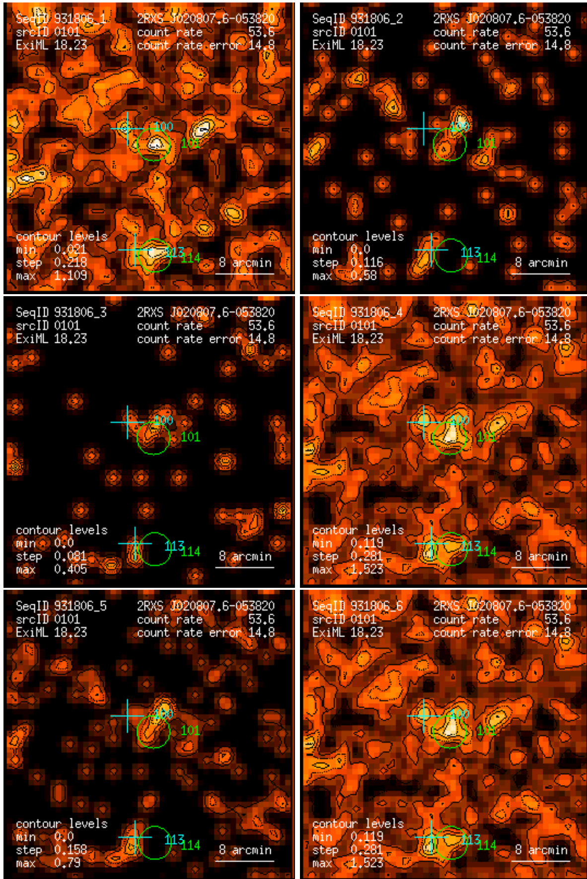
Figure 101: RASS 931806: detection 0101: band rate images, Gaussian filter: (1) PSPC channels 11 – 41, (2) 52 – 90, (3) 91 – 201, (4) 11 – 235, (5) 52 – 201, (6) 11 – 201. Broad band rates in counts/ks. Band rate contour levels in counts/ks/arcmin 2 .
