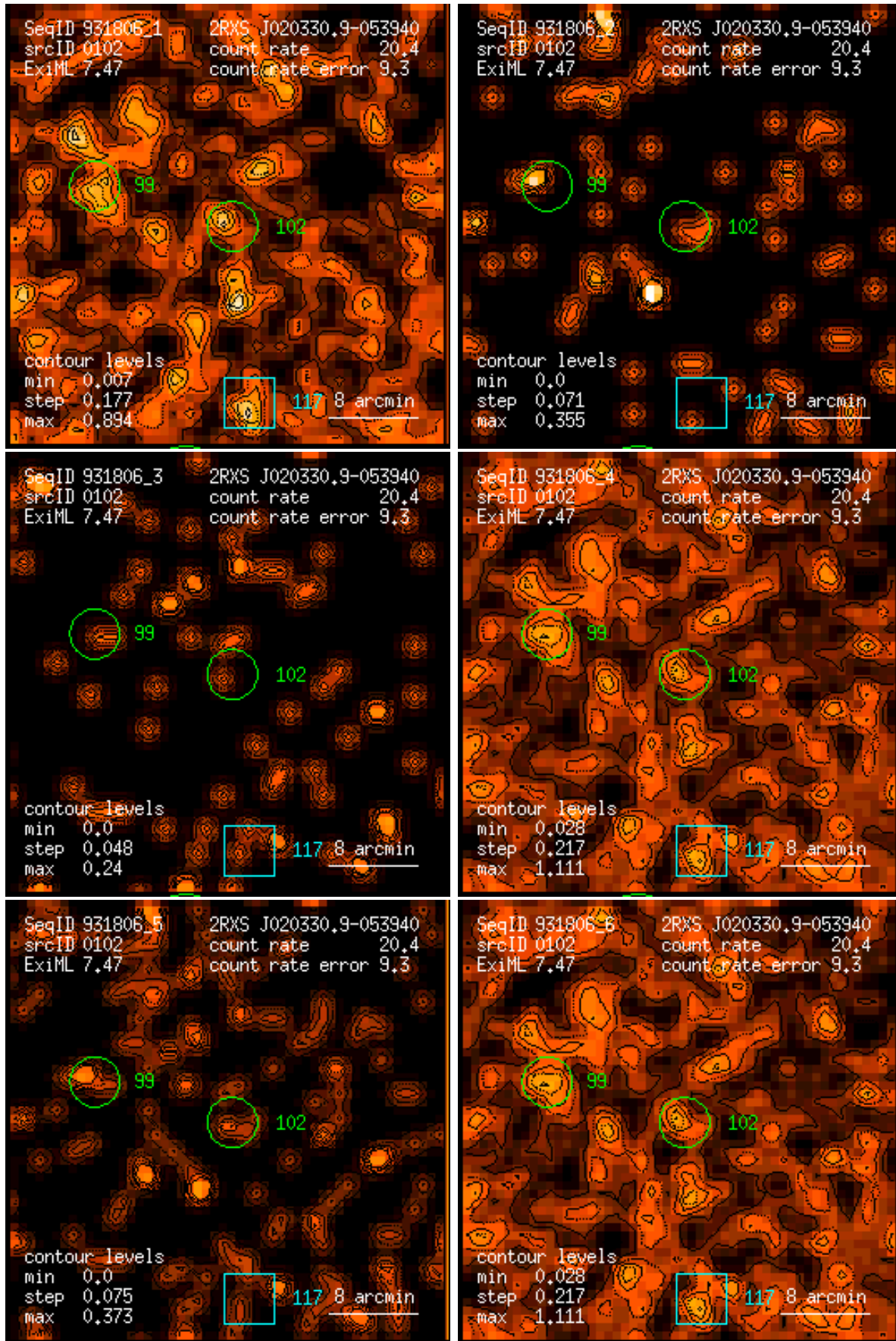
Figure 102: RASS 931806: detection 0102: band rate images, Gaussian filter: (1) PSPC channels 11 – 41, (2) 52 – 90, (3) 91 – 201, (4) 11 – 235, (5) 52 – 201, (6) 11 – 201. Broad band rates in counts/ks. Band rate contour levels in counts/ks/arcmin 2 .
