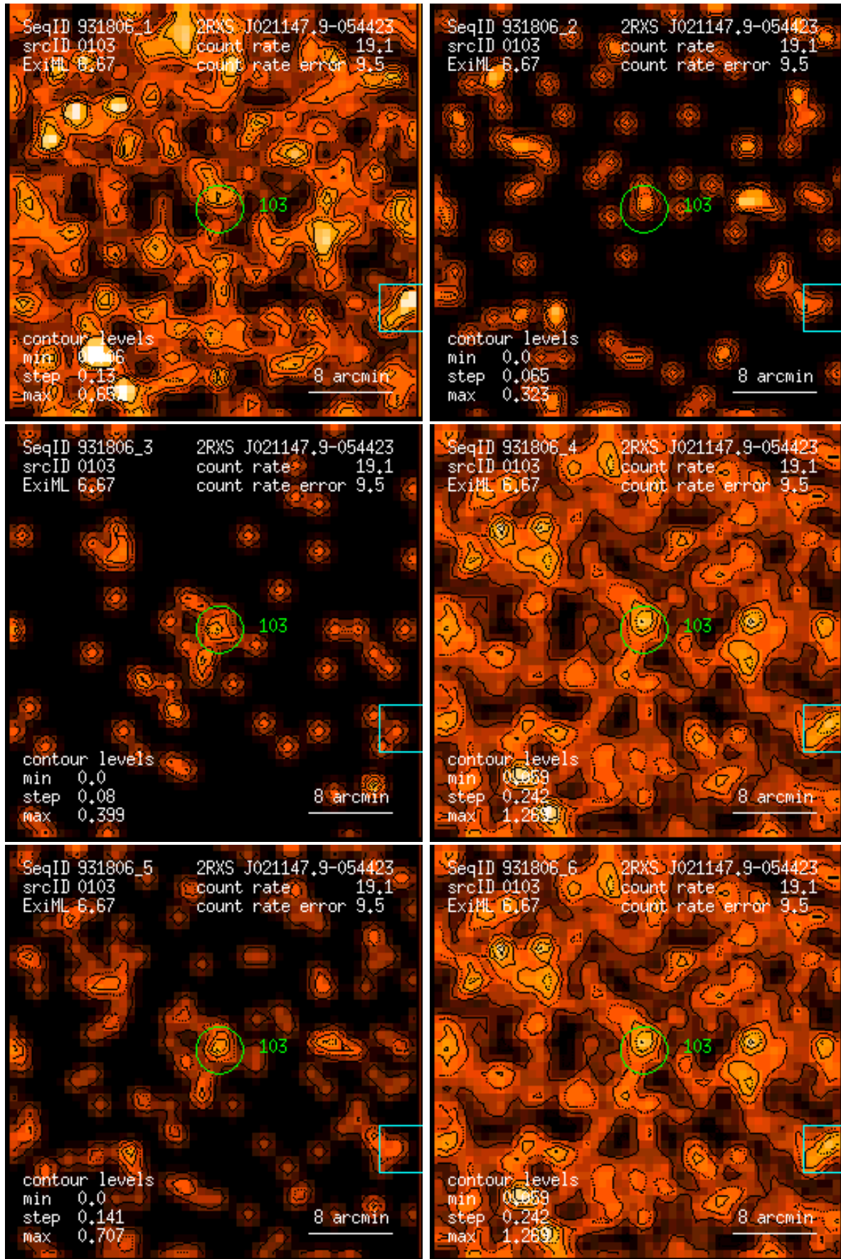
Figure 103: RASS 931806: detection 0103: band rate images, Gaussian filter: (1) PSPC channels 11 – 41, (2) 52 – 90, (3) 91 – 201, (4) 11 – 235, (5) 52 – 201, (6) 11 – 201. Broad band rates in counts/ks. Band rate contour levels in counts/ks/arcmin 2 .
