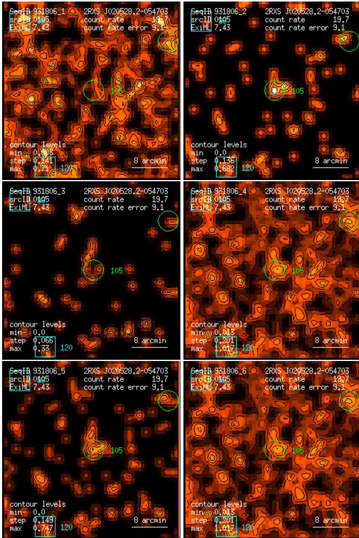
Figure 105: RASS 931806: detection 0105: band rate images, Gaussian filter: (1) PSPC channels 11 – 41, (2) 52 – 90, (3) 91 – 201, (4) 11 – 235, (5) 52 – 201, (6) 11 – 201. Broad band rates in counts/ks. Band rate contour levels in counts/ks/arcmin 2 .
