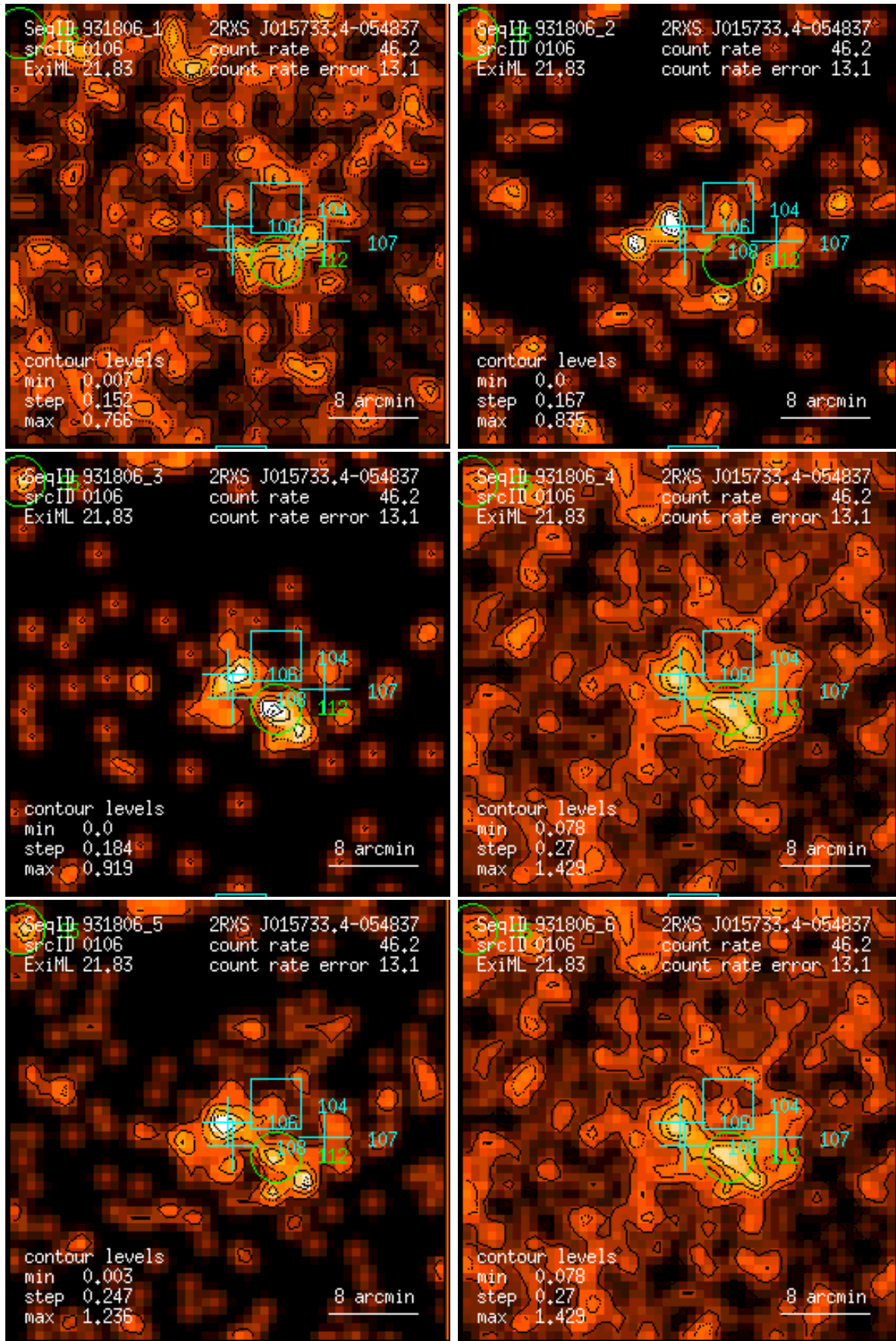
Figure 106: RASS 931806: detection 0106: band rate images, Gaussian filter: (1) PSPC channels 11 – 41, (2) 52 – 90, (3) 91 – 201, (4) 11 – 235, (5) 52 – 201, (6) 11 – 201. Broad band rates in counts/ks. Band rate contour levels in counts/ks/arcmin 2 .
