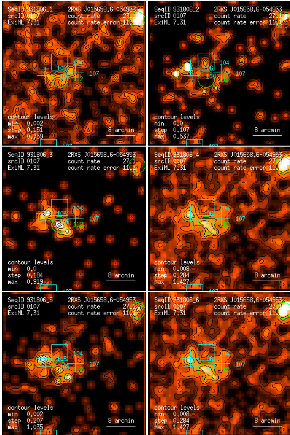
Figure 107: RASS 931806: detection 0107: band rate images, Gaussian filter: (1) PSPC channels 11 – 41, (2) 52 – 90, (3) 91 – 201, (4) 11 – 235, (5) 52 – 201, (6) 11 – 201. Broad band rates in counts/ks. Band rate contour levels in counts/ks/arcmin 2 .
