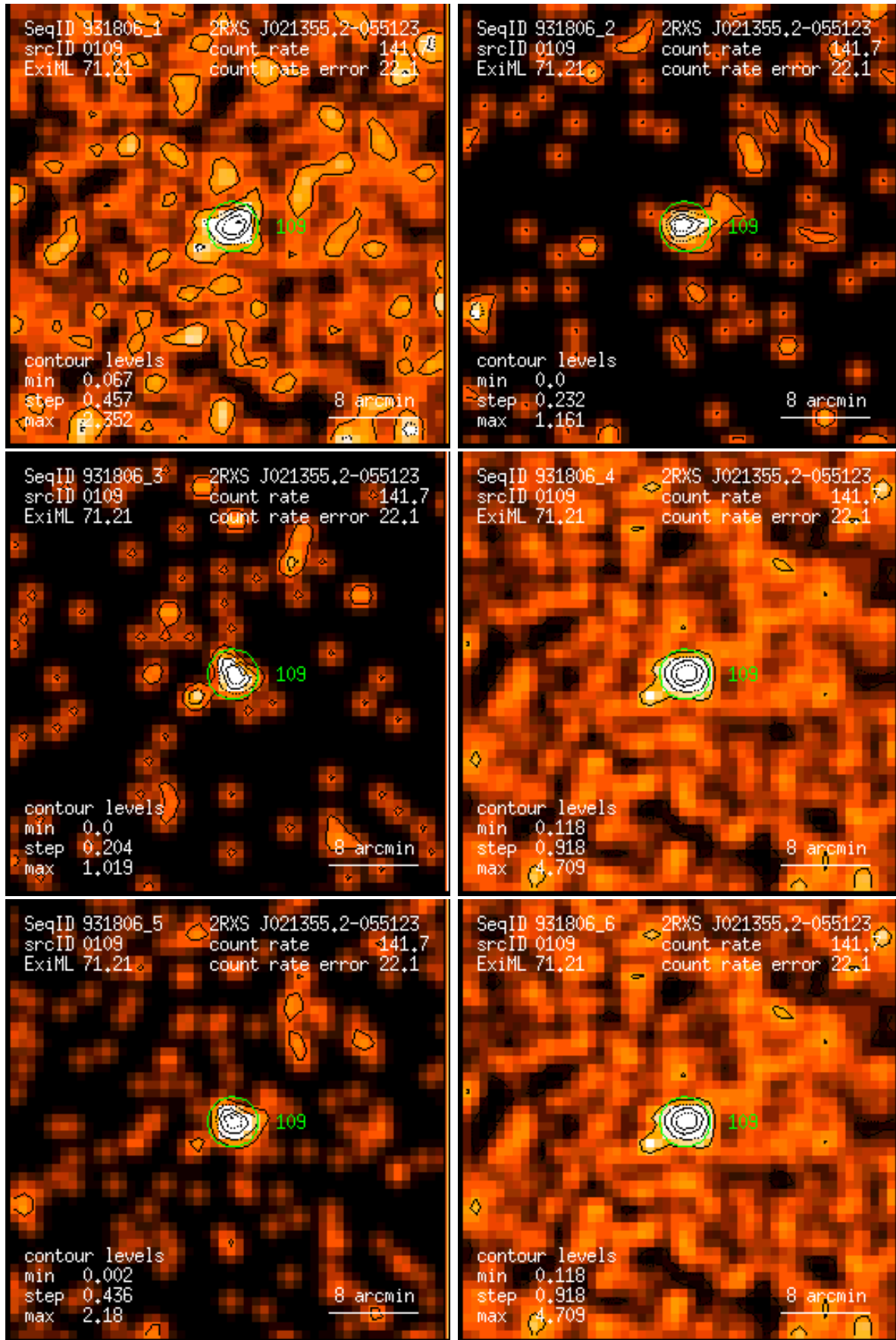
Figure 109: RASS 931806: detection 0109: band rate images, Gaussian filter: (1) PSPC channels 11 – 41, (2) 52 – 90, (3) 91 – 201, (4) 11 – 235, (5) 52 – 201, (6) 11 – 201. Broad band rates in counts/ks. Band rate contour levels in counts/ks/arcmin 2 .
