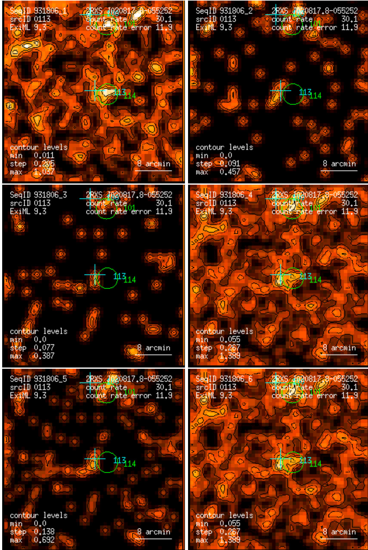
Figure 113: RASS 931806: detection 0113: band rate images, Gaussian filter: (1) PSPC channels 11 – 41, (2) 52 – 90, (3) 91 – 201, (4) 11 – 235, (5) 52 – 201, (6) 11 – 201. Broad band rates in counts/ks. Band rate contour levels in counts/ks/arcmin 2 .
