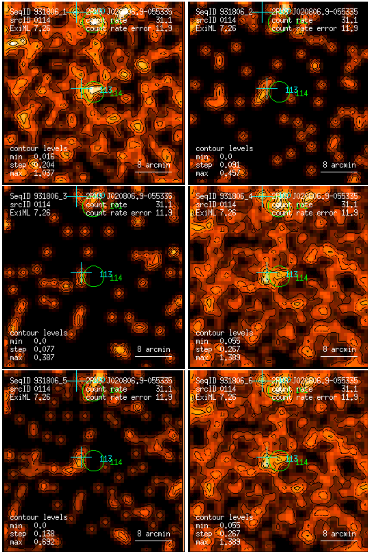
Figure 114: RASS 931806: detection 0114: band rate images, Gaussian filter: (1) PSPC channels 11 – 41, (2) 52 – 90, (3) 91 – 201, (4) 11 – 235, (5) 52 – 201, (6) 11 – 201. Broad band rates in counts/ks. Band rate contour levels in counts/ks/arcmin 2 .
